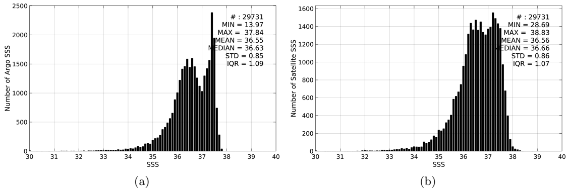
Figure 2: Histograms of SSS from Argo (a) and SMOS-L3-CATDS-CECOS-LOCEAN-V2-9DAYS-25KM (b) considering all match-up pairs per bins of 0.1 over the Amazon and Orinoco river plumes Pi-MEP region and for the full satellite product period.
