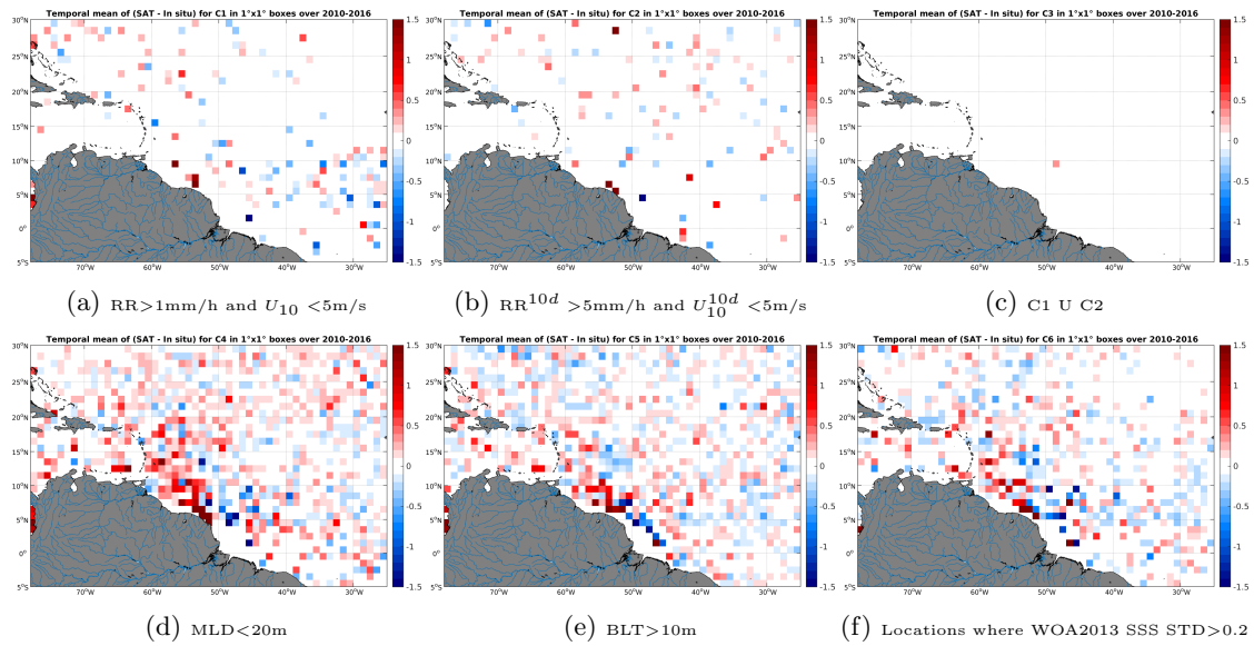
Figure 12: Temporal mean gridded over spatial boxes of size 1^\circ \times 1^\circ of \Delta SSS (SMOS-L3-CATDS-CECOS-LOCEAN-V2-9DAYS-25KM - Argo) for 6 different subdatasets corresponding to: RR > 1\text{mm/h} and U_{10} < 5\text{m/s} (a), RR^{10d} > 5\text{mm/h} and U_{10}^{10d} < 5\text{m/s} (b), C1 U C2 (c), MLD < 20\text{m} (d), BLT > 10\text{m} (e), Locations where WOA2013 SSS STD > 0.2 (f).
