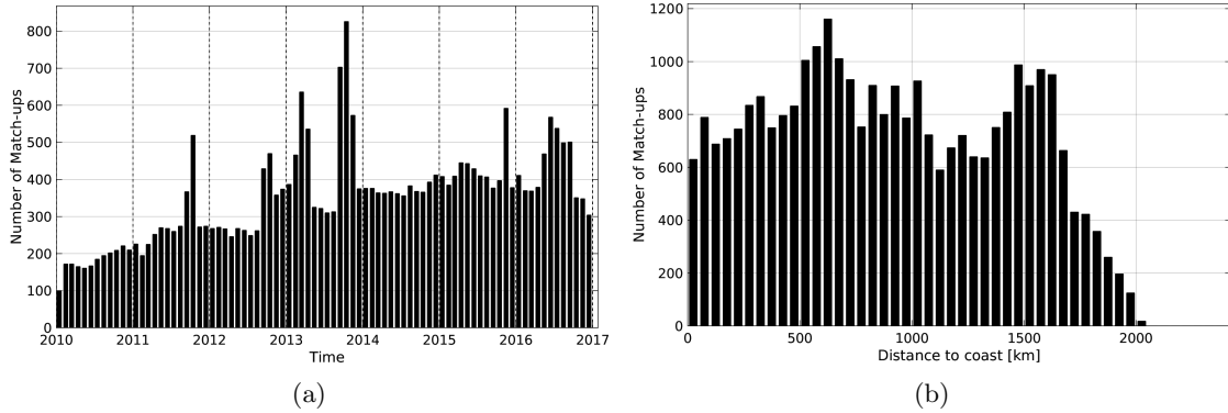
Figure 1: Number of match-ups between Argo and SMOS-L3-CATDS-CECOS-LOCEAN-V2-9DAYS-25KM SSS as a function of time (a) and as function of the distance to coast (b) over the Amazon and Orinoco river plumes Pi-MEP region and for the full satellite product period.
