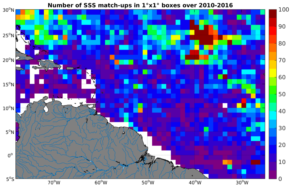
Figure 4: Number of SSS match-ups between Argo SSS and the SMOS-L3-CATDS-CECOS-LOCEAN-V2-9DAYS-25KM SSS product for the Amazon and Orinoco river plumes Pi-MEP region over 1°x1° boxes and for the full satellite product period.
