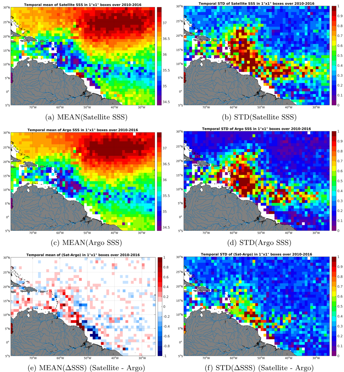
Figure 6: Temporal mean (left) and STD (right) of SSS from SMOS-L3-CATDS-CECOS-LOCEAN-V2-9DAYS-25KM (top), Argo (middle), and of \Delta SSS (Satellite - Argo). Only match-up pairs are used to generate these maps.
