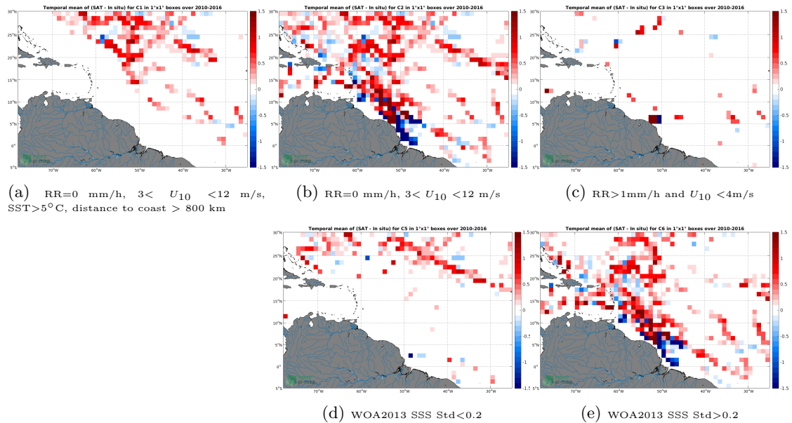
Figure 12: Temporal mean gridded over spatial boxes of size 1^{\circ}\times 1^{\circ} of \Delta\text{SSS} (SMOS SSS L3 v2 - Monthly - 0.25 Deg (CATDS-CECOS-IFREMER) - TSG (SAMOS)) for 5 different subdatasets corresponding to:RR=0 mm/h, 3 < U_{10} < 12 m/s, SST >5^{\circ}\text{C} , distance to coast > 800 km (a), RR=0 mm/h, 3 < U_{10} < 12 m/s (b), RR >1 mm/h and U_{10} < 4 m/s (c), WOA2013 SSS Std <0.2 (d), WOA2013 SSS Std >0.2 (e).
