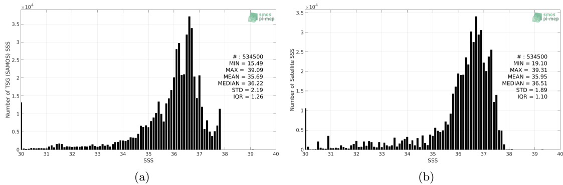
Figure 2: Histograms of SSS from TSG (SAMOS) (a) and SMOS SSS L3 v2 - Monthly - 0.25 Deg (CATDS-CECOS-IFREMER) (b) considering all match-up pairs per bins of 0.1 over the Amazon and Orinoco river plumes Pi-MEP region and for the full satellite product period.
