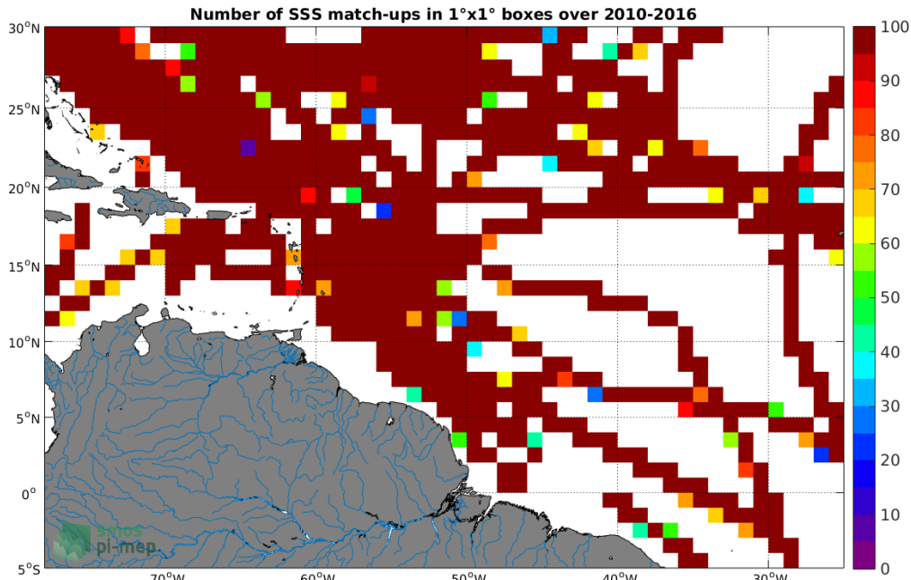
Figure 4: Number of SSS match-ups between TSG (SAMOS) SSS and the SMOS SSS L3 v2 - Monthly - 0.25 Deg (CATDS-CECOS-IFREMER) SSS product for the Amazon and Orinoco river plumes Pi-MEP region over 1^\circ \times 1^\circ boxes and for the full satellite product period.
