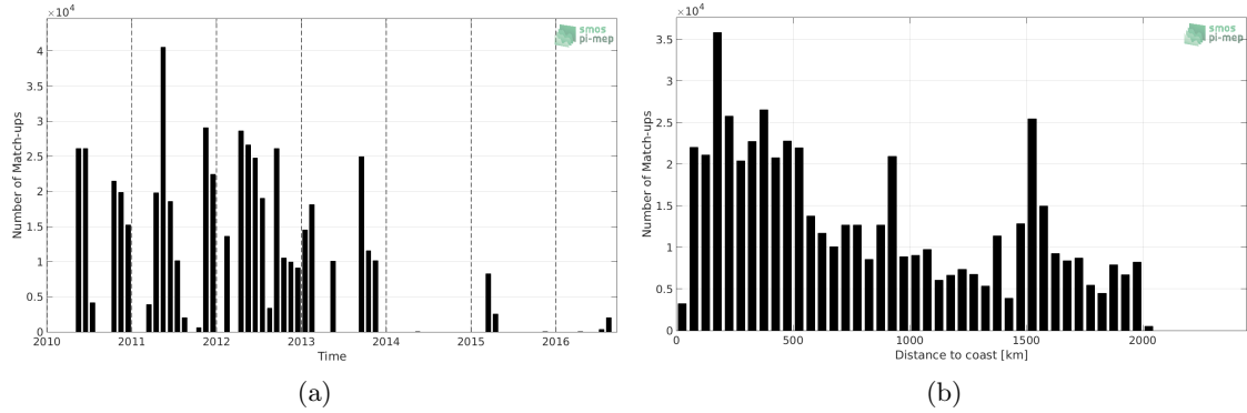
Figure 1: Number of match-ups between TSG (SAMOS) and SMOS SSS L3 v2 - Monthly - 0.25 Deg (CATDS-CECOS-IFREMER) SSS as a function of time (a) and as function of the distance to coast (b) over the Amazon and Orinoco river plumes Pi-MEP region and for the full satellite product period.
