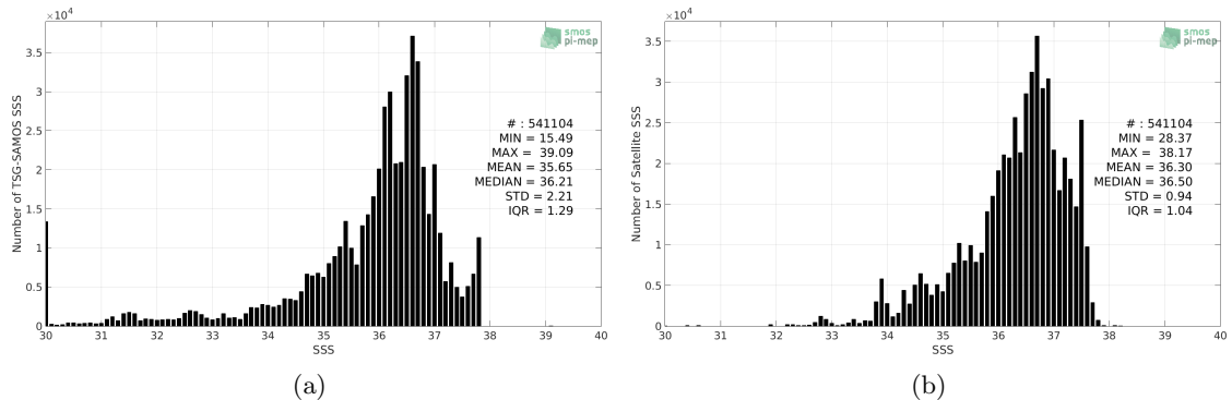
Figure 2: Histograms of SSS from TSG-SAMOS (a) and SMOS-L3-CATDS-IFREMER-CECOS-V2-MONTHLY-0.25DEG (b) considering all match-up pairs per bins of 0.1 over the Amazon and Orinoco river plumes Pi-MEP region and for the full satellite product period.
