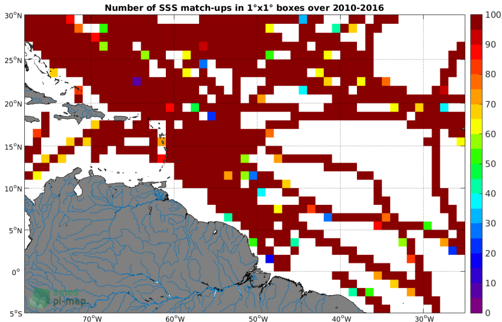
Figure 4: Number of SSS match-ups between TSG-SAMOS SSS and the SMOS-L3-CATDS-IFREMER-CECOS-V2-MONTHLY-0.25DEG SSS product for the Amazon and Orinoco river plumes Pi-MEP region over 1°x1° boxes and for the full satellite product period.
