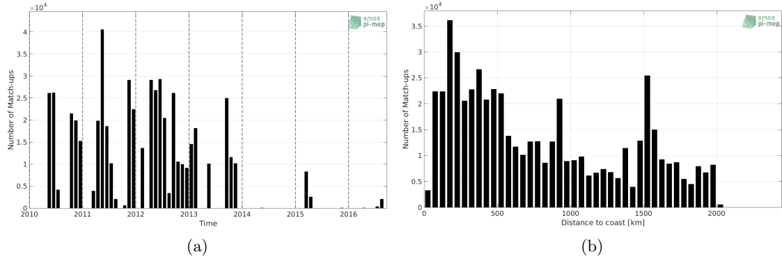
Figure 1: Number of match-ups between TSG-SAMOS and SMOS-L3-CATDS-IFREMER-CECOS-V2-MONTHLY-0.25DEG SSS as a function of time (a) and as function of the distance to coast (b) over the Amazon and Orinoco river plumes Pi-MEP region and for the full satellite product period.
