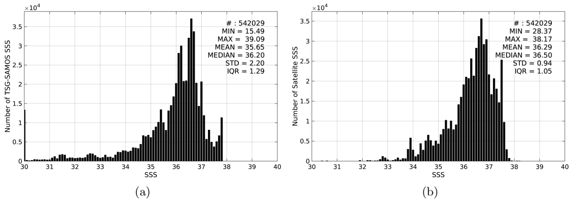
Figure 2: Histograms of SSS from TSG-SAMOS (a) and SMOS-L3-CATDS-IFREMER-CECOS-V2-MONTHLY-0.25DEG (b) considering all match-up pairs per bins of 0.1 over the Amazon and Orinoco river plumes Pi-MEP region and for the full satellite product period.
