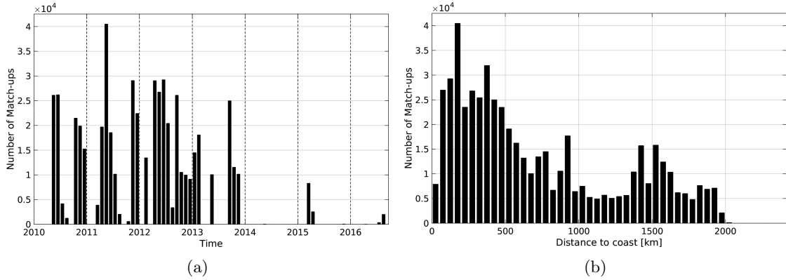
Figure 1: Number of match-ups between TSG-SAMOS and SMOS-L3-CATDS-IFREMER-CECOS-V2-MONTHLY-0.25DEG SSS as a function of time (a) and as function of the distance to coast (b) over the Amazon and Orinoco river plumes Pi-MEP region and for the full satellite product period.
