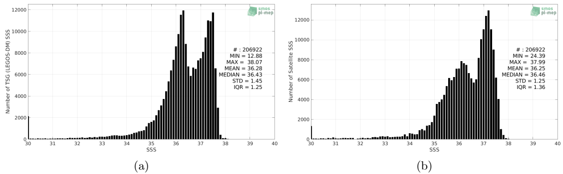
Figure 2: Histograms of SSS from TSG (LEGOS-DM) (a) and SMOS SSS L3 v2 - Monthly - 0.25 Deg (CATDS-CECOS-IFREMER) (b) considering all match-up pairs per bins of 0.1 over the Amazon and Orinoco river plumes Pi-MEP region and for the full satellite product period.
