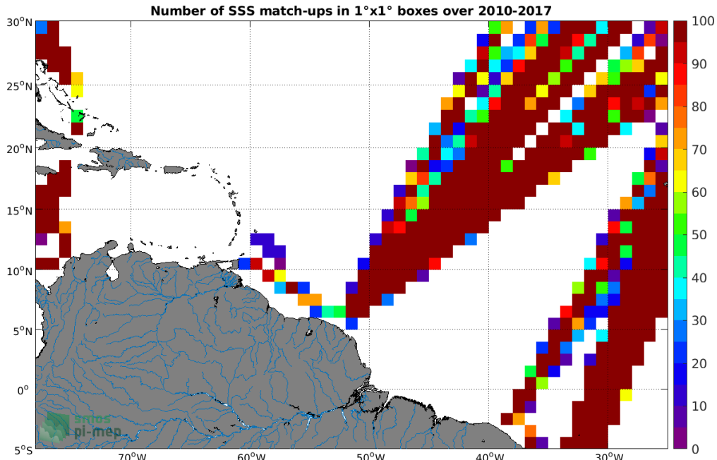
Figure 4: Number of SSS match-ups between TSG (LEGOS-DM) SSS and the SMOS SSS L3 v2 - Monthly - 0.25 Deg (CATDS-CECOS-IFREMER) SSS product for the Amazon and Orinoco river plumes Pi-MEP region over 1^\circ \times 1^\circ boxes and for the full satellite product period.
