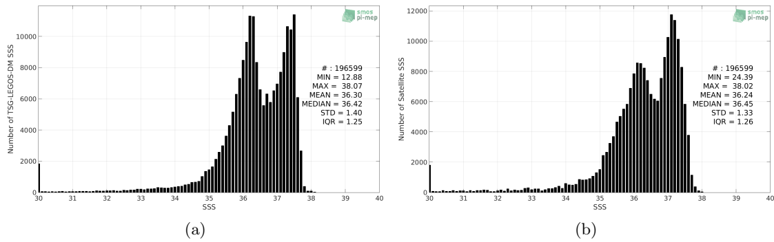
Figure 2: Histograms of SSS from TSG-LEGOS-DM (a) and SMOS L3 v2 - Monthly - 0.25 Deg (CATDS-CECOS-IFREMER) (b) considering all match-up pairs per bins of 0.1 over the Amazon and Orinoco river plumes Pi-MEP region and for the full satellite product period.
