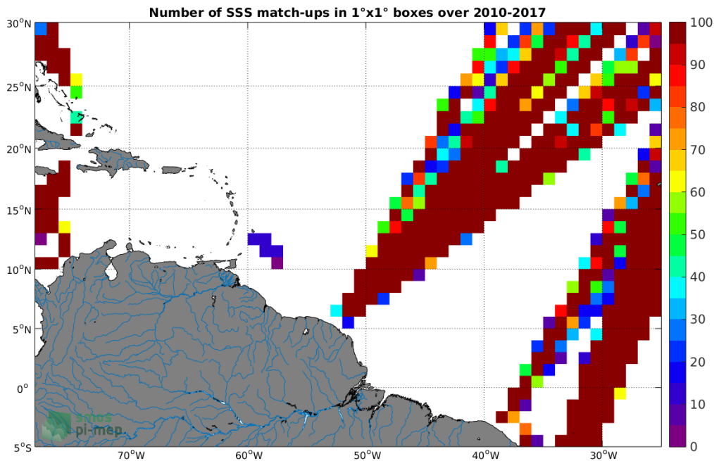
Figure 4: Number of SSS match-ups between TSG-LEGOS-DM SSS and the SMOS L3 v2 - Monthly - 0.25 Deg (CATDS-CECOS-IFREMER) SSS product for the Amazon and Orinoco river plumes Pi-MEP region over 1°x1° boxes and for the full satellite product period.
