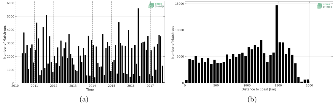
Figure 1: Number of match-ups between TSG-LEGOS-DM and SMOS L3 v2 - Monthly - 0.25 Deg (CATDS-CECOS-IFREMER) SSS as a function of time (a) and as function of the distance to coast (b) over the Amazon and Orinoco river plumes Pi-MEP region and for the full satellite product period.
