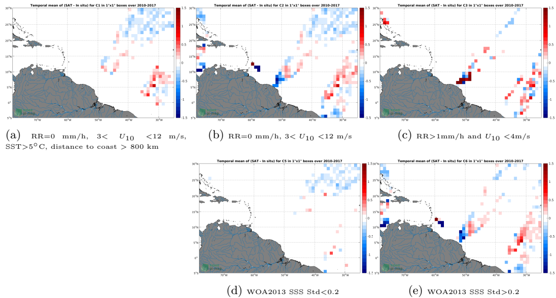
Figure 12: Temporal mean gridded over spatial boxes of size 1^{\circ}\times 1^{\circ} of \Delta\text{SSS} (SMOS L3 v2 - Monthly - 0.25 Deg (CATDS-CECOS-IFREMER) - TSG-LEGOS-DM) for 5 different subdatasets corresponding to:RR=0 mm/h, 3 < U_{10} < 12 m/s, SST >5^{\circ}\text{C} , distance to coast > 800 km (a), RR=0 mm/h, 3 < U_{10} < 12 m/s (b), RR >1 mm/h and U_{10} < 4 m/s (c), WOA2013 SSS Std <0.2 (d), WOA2013 SSS Std >0.2 (e).
