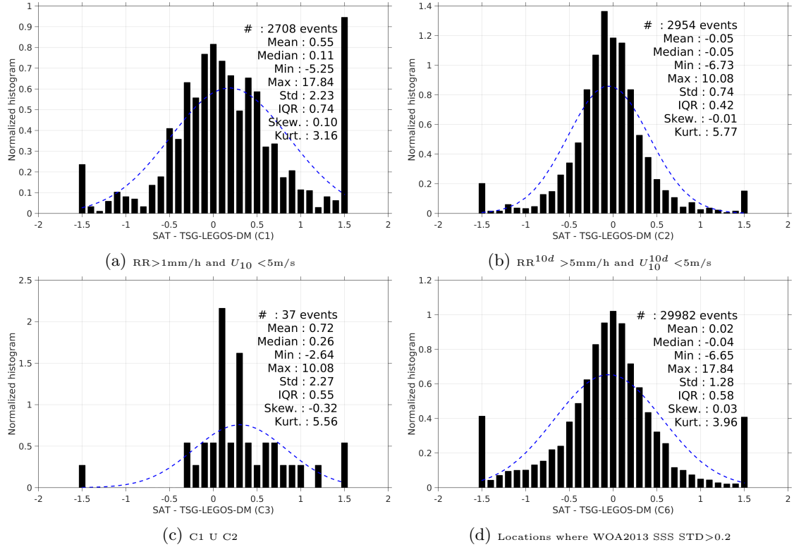
Figure 13: Normalized histogram of \Delta SSS (SMOS-L3-CATDS-IFREMER-CECOS-V2-MONTHLY-0.25DEG - TSG-LEGOS-DM) for 6 different subdatasets corresponding to: RR > 1\text{mm/h} and U_{10} < 5\text{m/s} (a), RR^{10d} > 5\text{mm/h} and U_{10}^{10d} < 5\text{m/s} (b), C1 U C2 (c), Locations where WOA2013 SSS STD > 0.2 (d).
