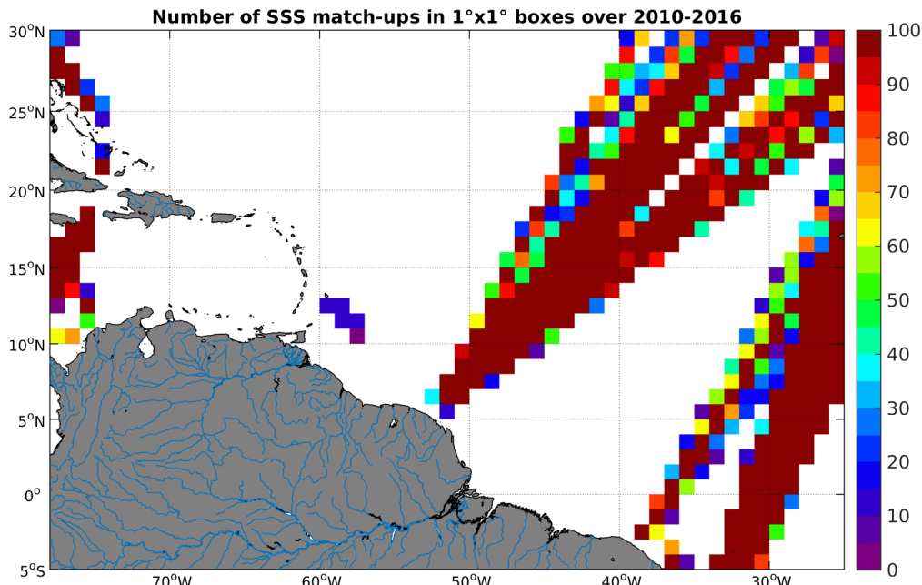
Figure 4: Number of SSS match-ups between TSG-LEGOS-DM SSS and the SMOS-L3-CATDS-IFREMER-CECOS-V2-MONTHLY-0.25DEG SSS product for the Amazon and Orinoco river plumes Pi-MEP region over 1^\circ \times 1^\circ boxes and for the full satellite product period.
