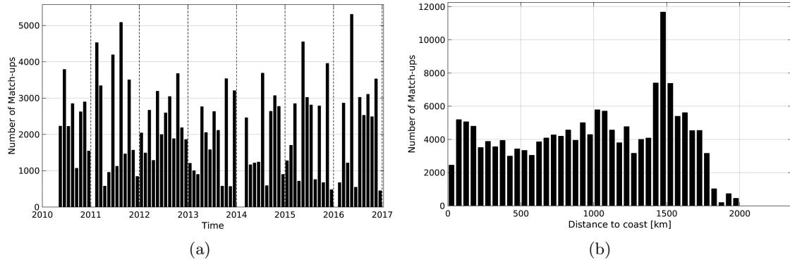
Figure 1: Number of match-ups between TSG-LEGOS-DM and SMOS-L3-CATDS-IFREMER-CECOS-V2-MONTHLY-0.25DEG SSS as a function of time (a) and as function of the distance to coast (b) over the Amazon and Orinoco river plumes Pi-MEP region and for the full satellite product period.
