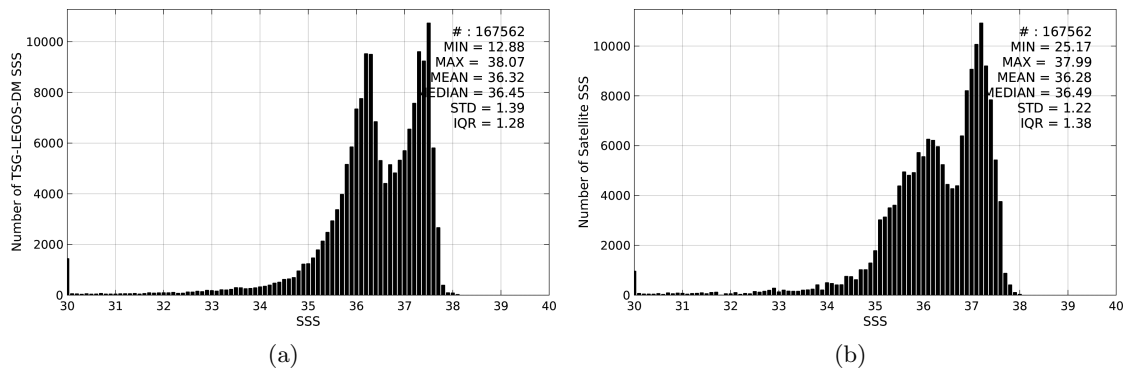
Figure 2: Histograms of SSS from TSG-LEGOS-DM (a) and SMOS-L3-CATDS-IFREMER-CECOS-V2-MONTHLY-0.25DEG (b) considering all match-up pairs per bins of 0.1 over the Amazon and Orinoco river plumes Pi-MEP region and for the full satellite product period.
