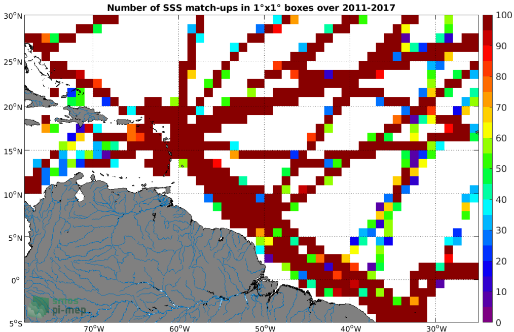
Figure 4: Number of SSS match-ups between TSG (GOSUD-Research-vessel) SSS and the SMOS SSS L3 v2 - Monthly - 0.25 Deg (CATDS-CECOS-IFREMER) SSS product for the Amazon and Orinoco river plumes Pi-MEP region over 1^\circ \times 1^\circ boxes and for the full satellite product period.
