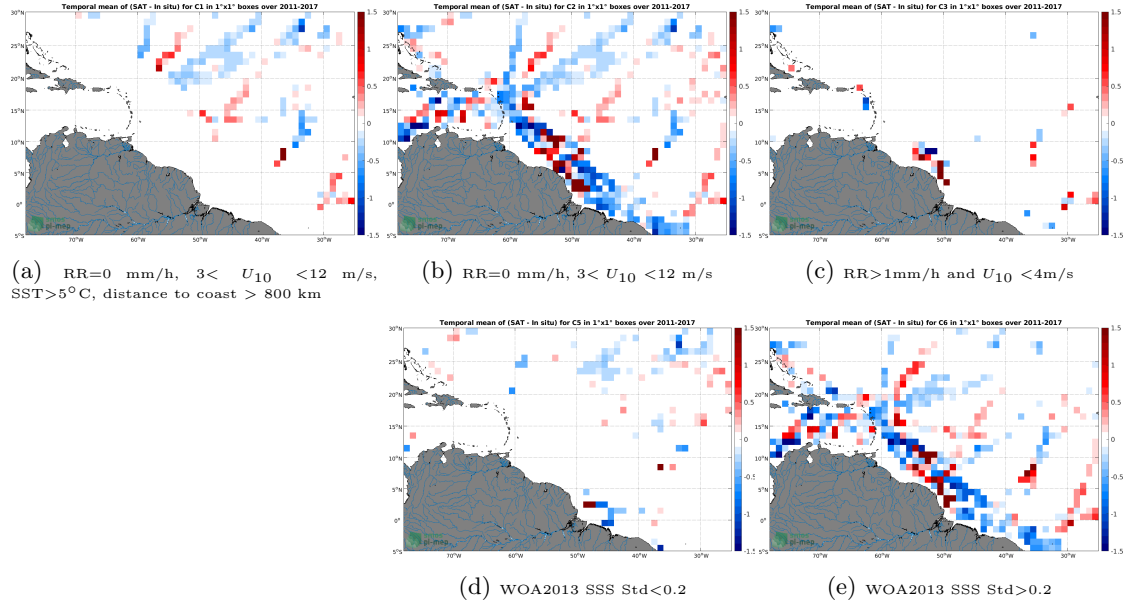
Figure 12: Temporal mean gridded over spatial boxes of size 1^{\circ}\times 1^{\circ} of \Delta SSS (SMOS SSS L3 v2 - Monthly - 0.25 Deg (CATDS-CECOS-IFREMER) - TSG (GOSUD-Research-vessel)) for 5 different subdatasets corresponding to:RR=0 mm/h, 3 < U_{10} < 12 m/s, SST >5^{\circ}\text{C} , distance to coast > 800 km (a), RR=0 mm/h, 3 < U_{10} < 12 m/s (b), RR >1 mm/h and U_{10} < 4 m/s (c), WOA2013 SSS Std <0.2 (d), WOA2013 SSS Std >0.2 (e).
