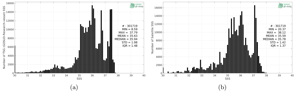
Figure 2: Histograms of SSS from TSG (GOSUD-Research-vessel) (a) and SMOS SSS L3 v2 - Monthly - 0.25 Deg (CATDS-CECOS-IFREMER) (b) considering all match-up pairs per bins of 0.1 over the Amazon and Orinoco river plumes Pi-MEP region and for the full satellite product period.
