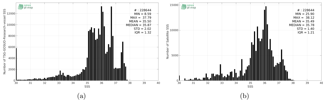
Figure 2: Histograms of SSS from TSG-GOSUD-Research-vessel (a) and SMOS-L3-CATDS-IFREMER-CECOS-V2-MONTHLY-0.25DEG (b) considering all match-up pairs per bins of 0.1 over the Amazon and Orinoco river plumes Pi-MEP region and for the full satellite product period.
