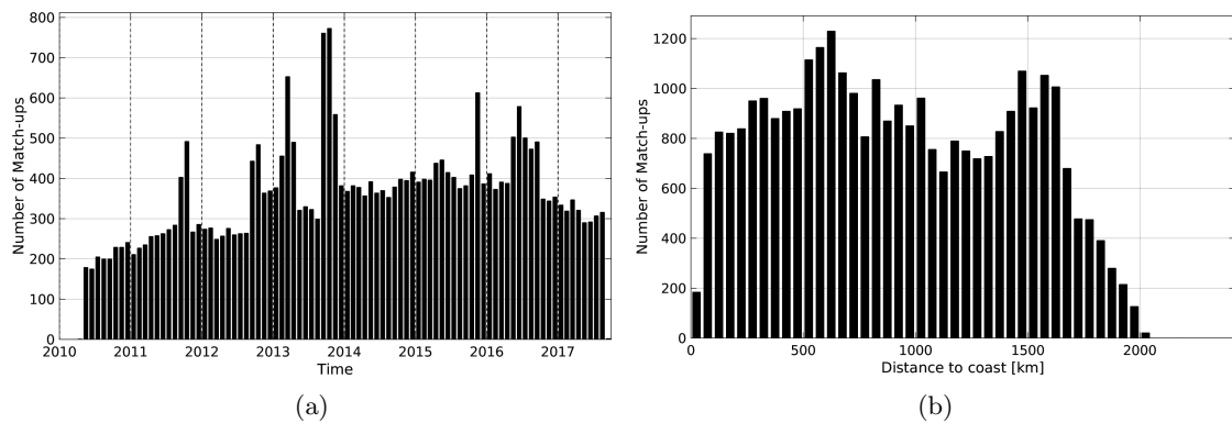
Figure 1: Number of match-ups between Argo and SMOS-L3-CATDS-IFREMER-CECOS-V2-MONTHLY-0.25DEG SSS as a function of time (a) and as function of the distance to coast (b) over the Amazon and Orinoco river plumes Pi-MEP region and for the full satellite product period.
