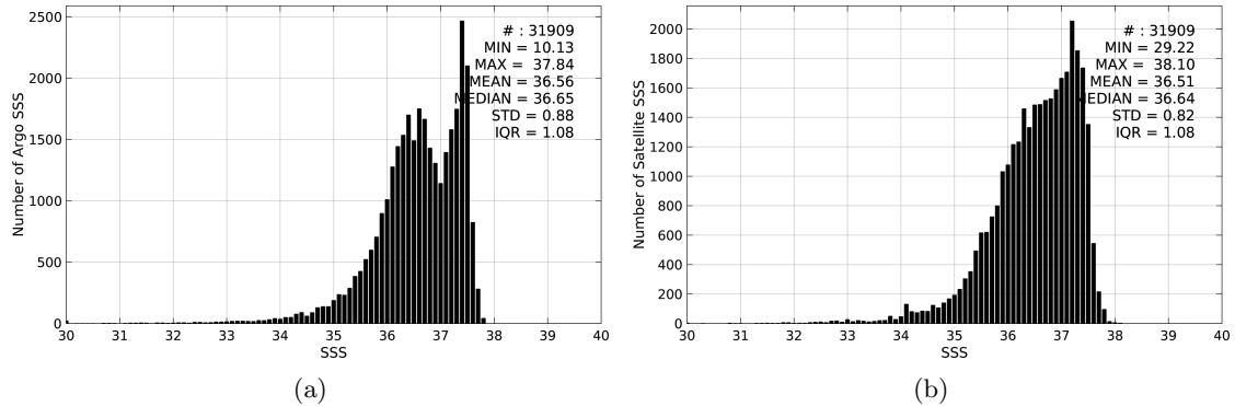
Figure 2: Histograms of SSS from Argo (a) and SMOS-L3-CATDS-IFREMER-CECOS-V2-MONTHLY-0.25DEG (b) considering all match-up pairs per bins of 0.1 over the Amazon and Orinoco river plumes Pi-MEP region and for the full satellite product period.
