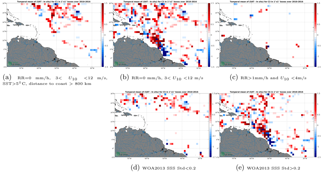
Figure 12: Temporal mean gridded over spatial boxes of size 1^{\circ}\times 1^{\circ} of \Delta\text{SSS} (SMOS SSS L3 v2 - Daily - 0.5 Deg (CATDS-CECOS-IFREMER) - TSG (SAMOS)) for 5 different subdatasets corresponding to: RR=0 mm/h, 3 < U_{10} < 12 m/s, SST > 5^{\circ}\text{C} , distance to coast > 800 km (a), RR=0 mm/h, 3 < U_{10} < 12 m/s (b), RR > 1 mm/h and U_{10} < 4 m/s (c), WOA2013 SSS Std < 0.2 (d), WOA2013 SSS Std > 0.2 (e).
