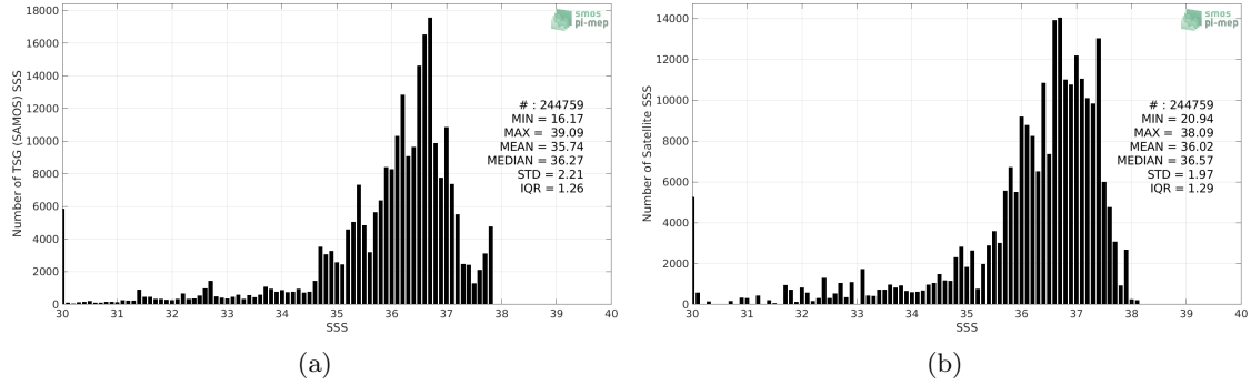
Figure 2: Histograms of SSS from TSG (SAMOS) (a) and SMOS SSS L3 v2 - Daily - 0.5 Deg (CATDS-CECOS-IFREMER) (b) considering all match-up pairs per bins of 0.1 over the Amazon and Orinoco river plumes Pi-MEP region and for the full satellite product period.
