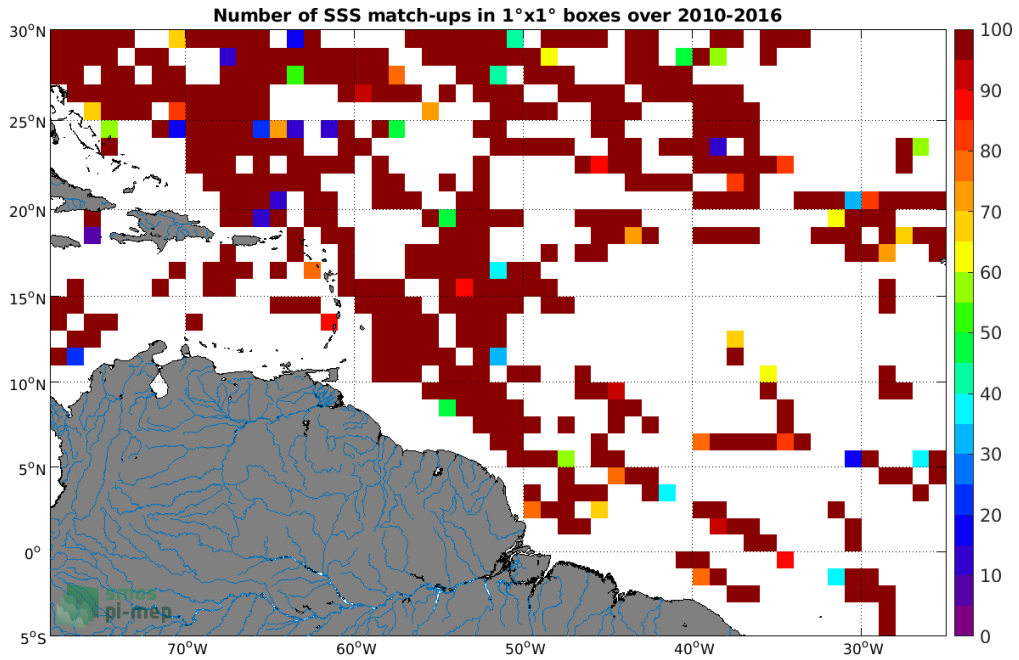
Figure 4: Number of SSS match-ups between TSG (SAMOS) SSS and the SMOS SSS L3 v2 - Daily - 0.5 Deg (CATDS-CECOS-IFREMER) SSS product for the Amazon and Orinoco river plumes Pi-MEP region over 1^\circ \times 1^\circ boxes and for the full satellite product period.
