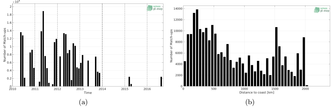
Figure 1: Number of match-ups between TSG (SAMOS) and SMOS SSS L3 v2 - Daily - 0.5 Deg (CATDS-CECOS-IFREMER) SSS as a function of time (a) and as function of the distance to coast (b) over the Amazon and Orinoco river plumes Pi-MEP region and for the full satellite product period.
