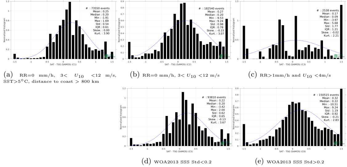
Figure 13: Normalized histogram of \Delta\text{SSS} (SMOS SSS L3 v2 - Daily - 0.5 Deg (CATDS-CECOS-IFREMER) - TSG (SAMOS)) for 5 different subdatasets corresponding to: RR=0 mm/h, 3 < U_{10} < 12 m/s, SST > 5^\circ\text{C} , distance to coast > 800 km (a), RR=0 mm/h, 3 < U_{10} < 12 m/s (b), RR > 1\text{mm/h} and U_{10} < 4\text{m/s} (c), WOA2013 SSS Std < 0.2 (d), WOA2013 SSS Std > 0.2 (e).
