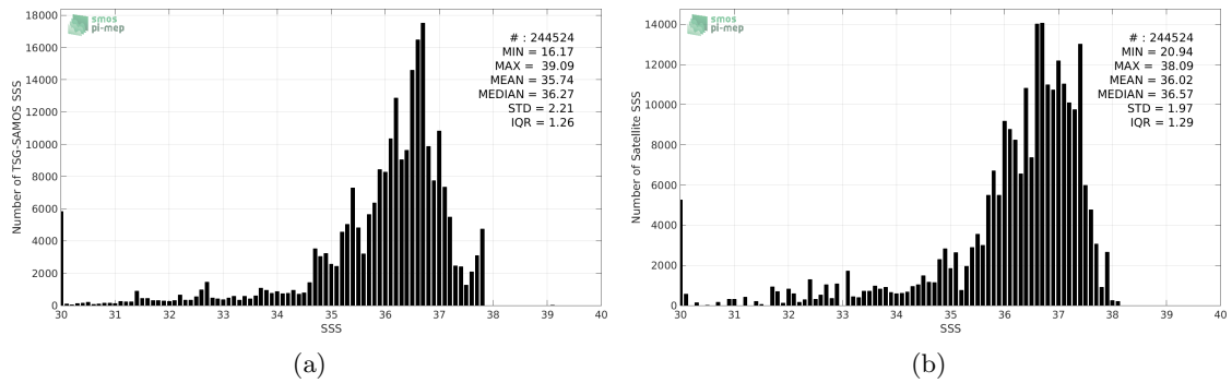
Figure 2: Histograms of SSS from TSG-SAMOS (a) and SMOS-L3-CATDS-CECOS-IFREMER-V2-1DAY-0.5DEG (b) considering all match-up pairs per bins of 0.1 over the Amazon and Orinoco river plumes Pi-MEP region and for the full satellite product period.
