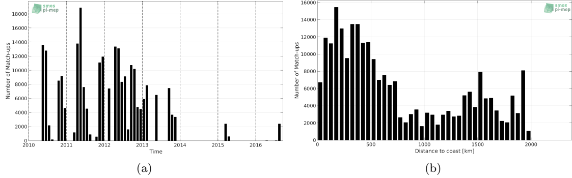
Figure 1: Number of match-ups between TSG-SAMOS and SMOS-L3-CATDS-CECOS-IFREMER-V2-1DAY-0.5DEG SSS as a function of time (a) and as function of the distance to coast (b) over the Amazon and Orinoco river plumes Pi-MEP region and for the full satellite product period.
