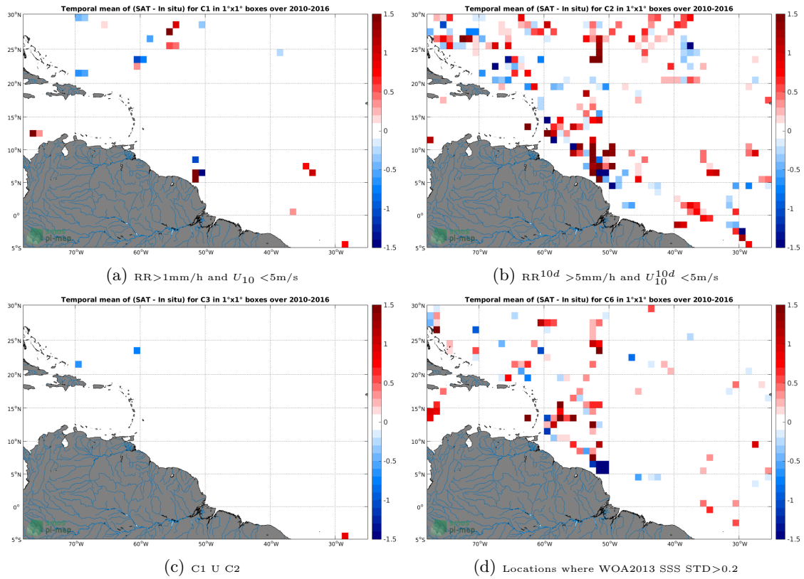
Figure 12: Temporal mean gridded over spatial boxes of size 1^\circ \times 1^\circ of \Delta SSS (SMOS-L3-CATDS-CECOS-IFREMER-V2-1DAY-0.5DEG - TSG-SAMOS) for 4 different subdatasets corresponding to: RR > 1\text{mm/h} and U_{10} < 5\text{m/s} (a), RR^{10d} > 5\text{mm/h} and U_{10}^{10d} < 5\text{m/s} (b), C1 U C2 (c), Locations where WOA2013 SSS STD > 0.2 (d).
