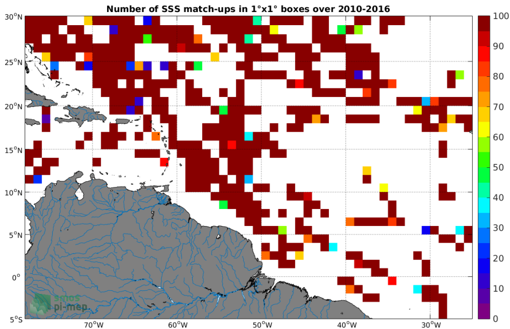
Figure 4: Number of SSS match-ups between TSG-SAMOS SSS and the SMOS-L3-CATDS-CECOS-IFREMER-V2-1DAY-0.5DEG SSS product for the Amazon and Orinoco river plumes Pi-MEP region over 1^\circ \times 1^\circ boxes and for the full satellite product period.
