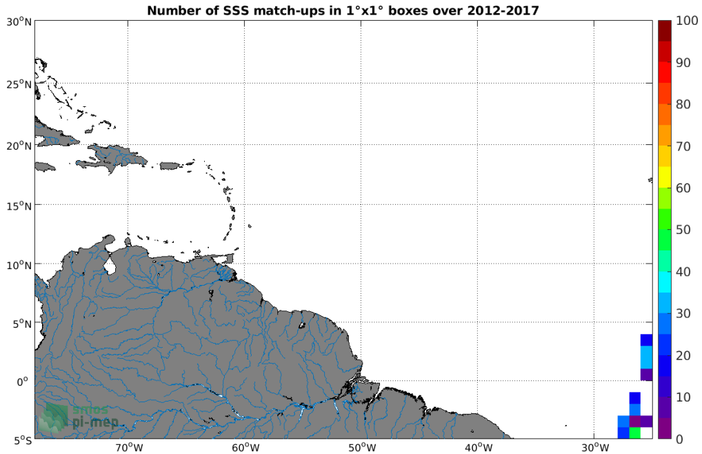
Figure 4: Number of SSS match-ups between TSG (Polarstern) SSS and the SMOS SSS L3 v2 - Daily - 0.5 Deg (CATDS-CECOS-IFREMER) SSS product for the Amazon and Orinoco river plumes Pi-MEP region over 1°x1° boxes and for the full satellite product period.
