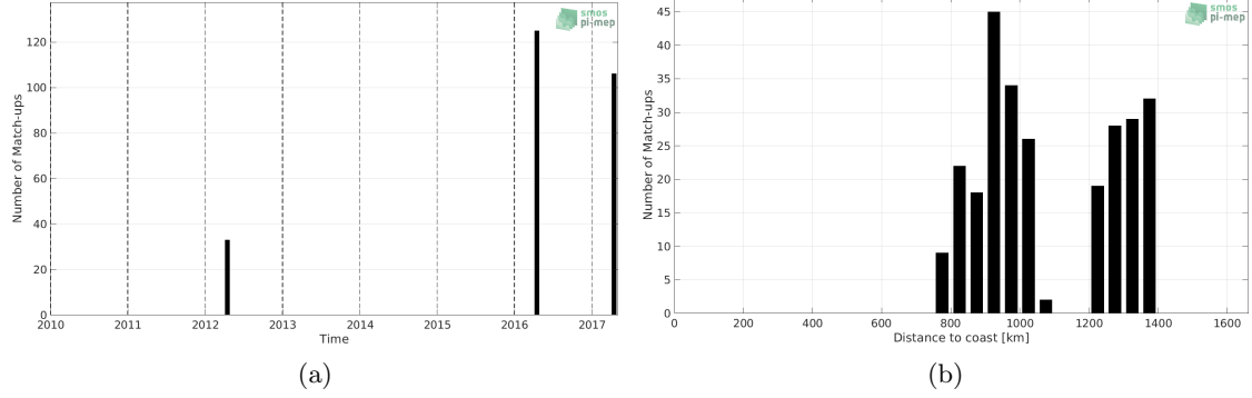
Figure 1: Number of match-ups between TSG (Polarstern) and SMOS SSS L3 v2 - Daily - 0.5 Deg (CATDS-CECOS-IFREMER) SSS as a function of time (a) and as function of the distance to coast (b) over the Amazon and Orinoco river plumes Pi-MEP region and for the full satellite product period.
