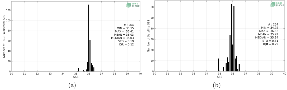
Figure 2: Histograms of SSS from TSG (Polarstern) (a) and SMOS SSS L3 v2 - Daily - 0.5 Deg (CATDS-CECOS-IFREMER) (b) considering all match-up pairs per bins of 0.1 over the Amazon and Orinoco river plumes Pi-MEP region and for the full satellite product period.
