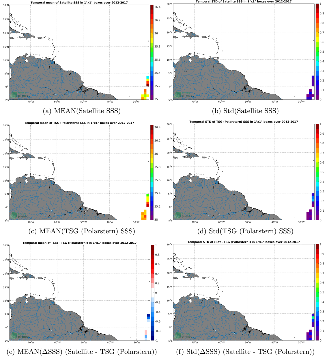
Figure 6: Temporal mean (left) and Std (right) of SSS from SMOS SSS L3 v2 - Daily - 0.5 Deg (CATDS-CECOS-IFREMER) (top), TSG (Polarstern) (middle), and of \Delta SSS (Satellite - TSG (Polarstern)). Only match-up pairs are used to generate these maps.
