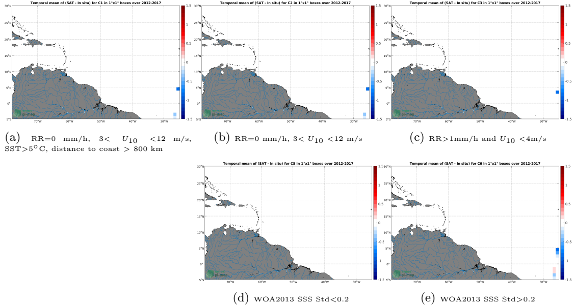
Figure 12: Temporal mean gridded over spatial boxes of size 1^{\circ}\times 1^{\circ} of \Delta\text{SSS} (SMOS SSS L3 v2 - Daily - 0.5 Deg (CATDS-CECOS-IFREMER) - TSG (Polarstern)) for 5 different subdatasets corresponding to:RR=0 mm/h, 3 < U_{10} < 12 m/s, SST >5^{\circ}\text{C} , distance to coast > 800 km (a), RR=0 mm/h, 3 < U_{10} < 12 m/s (b), RR >1 mm/h and U_{10} < 4 m/s (c), WOA2013 SSS Std <0.2 (d), WOA2013 SSS Std >0.2 (e).
