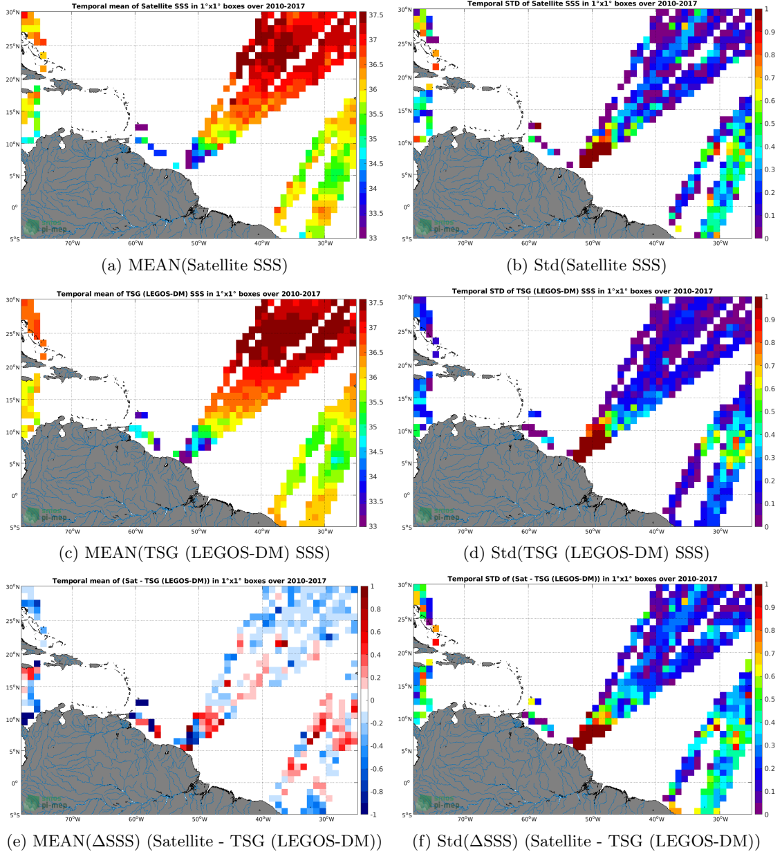
Figure 6: Temporal mean (left) and Std (right) of SSS from SMOS SSS L3 v2 - Daily - 0.5 Deg (CATDS-CECOS-IFREMER) (top), TSG (LEGOS-DM) (middle), and of \Delta SSS (Satellite - TSG (LEGOS-DM)). Only match-up pairs are used to generate these maps.
