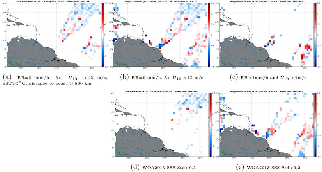
Figure 12: Temporal mean gridded over spatial boxes of size 1^{\circ}\times 1^{\circ} of \Delta\text{SSS} (SMOS SSS L3 v2 - Daily - 0.5 Deg (CATDS-CECOS-IFREMER) - TSG (LEGOS-DM)) for 5 different subdatasets corresponding to:RR=0 mm/h, 3 < U_{10} < 12 m/s, SST >5^{\circ}\text{C} , distance to coast > 800 km (a), RR=0 mm/h, 3 < U_{10} < 12 m/s (b), RR >1 mm/h and U_{10} < 4 m/s (c), WOA2013 SSS Std <0.2 (d), WOA2013 SSS Std >0.2 (e).
