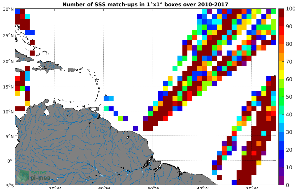
Figure 4: Number of SSS match-ups between TSG (LEGOS-DM) SSS and the SMOS SSS L3 v2 - Daily - 0.5 Deg (CATDS-CECOS-IFREMER) SSS product for the Amazon and Orinoco river plumes Pi-MEP region over 1^\circ \times 1^\circ boxes and for the full satellite product period.
