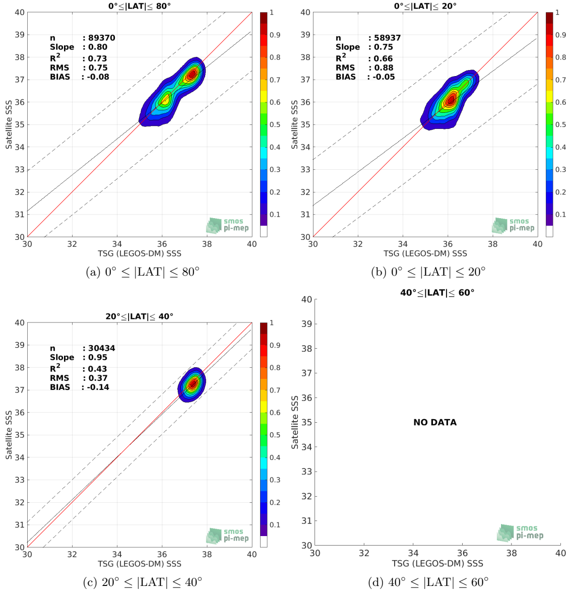
Figure 9: Contour maps of the concentration of SMOS SSS L3 v2 - Daily - 0.5 Deg (CATDS-CECOS-IFREMER) SSS (y-axis) versus TSG (LEGOS-DM) SSS (x-axis) at match-up pairs for different latitude bands. For each plot, the red line shows x=y . The black thin and dashed lines indicate a linear fit through the data cloud and the \pm 95\% confidence levels, respectively. The number match-up pairs n , the slope and R^2 coefficient of the linear fit, the root mean square (RMS) and the mean bias between satellite and in situ data are indicated for each latitude band in each plots.
