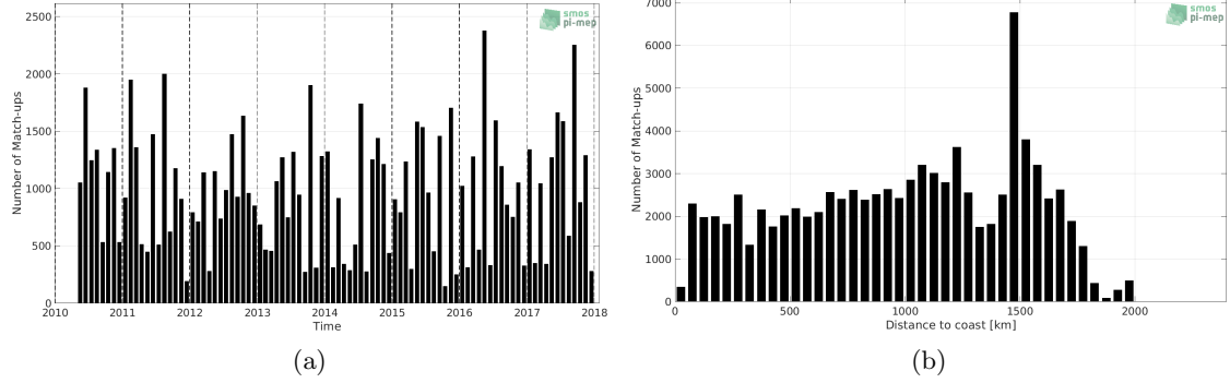
Figure 1: Number of match-ups between TSG (LEGOS-DM) and SMOS SSS L3 v2 - Daily - 0.5 Deg (CATDS-CECOS-IFREMER) SSS as a function of time (a) and as function of the distance to coast (b) over the Amazon and Orinoco river plumes Pi-MEP region and for the full satellite product period.
