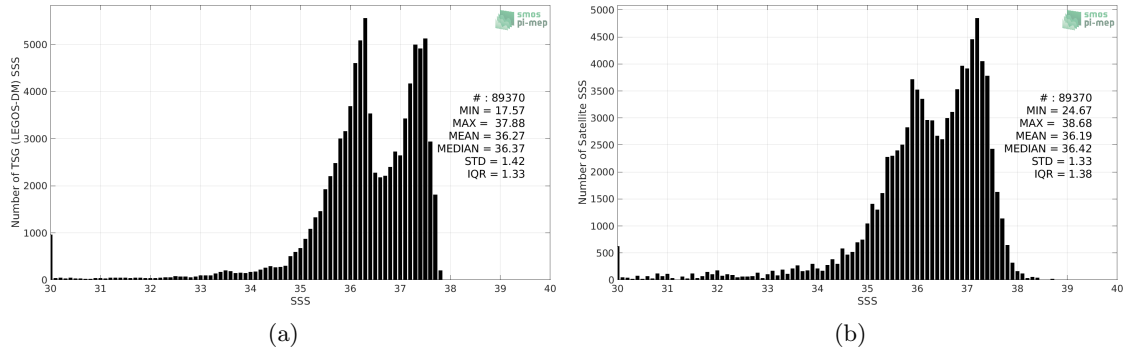
Figure 2: Histograms of SSS from TSG (LEGOS-DM) (a) and SMOS SSS L3 v2 - Daily - 0.5 Deg (CATDS-CECOS-IFREMER) (b) considering all match-up pairs per bins of 0.1 over the Amazon and Orinoco river plumes Pi-MEP region and for the full satellite product period.
