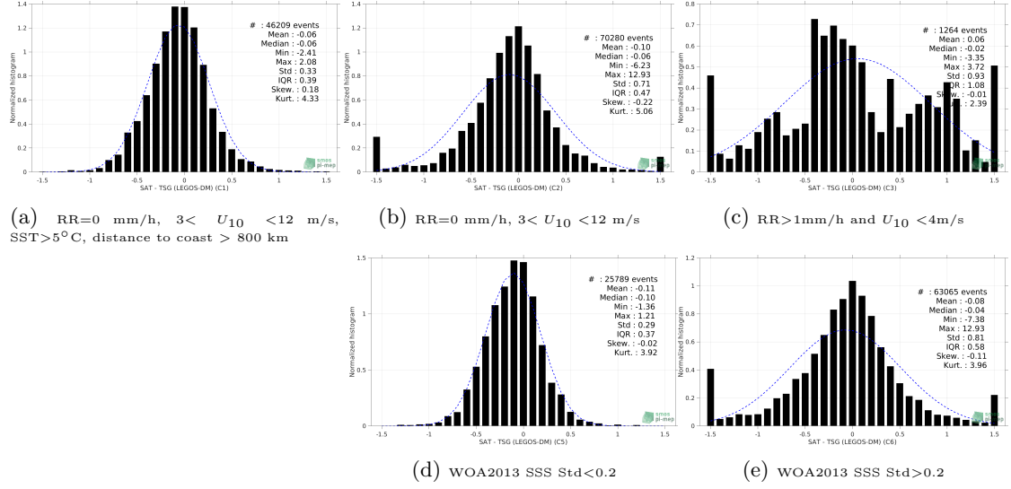
Figure 13: Normalized histogram of \Delta SSS (SMOS SSS L3 v2 - Daily - 0.5 Deg (CATDS-CECOS-IFREMER) - TSG (LEGOS-DM)) for 5 different subdatasets corresponding to: RR=0 mm/h, 3 < U_{10} < 12 m/s, SST>5°C, distance to coast > 800 km (a), RR=0 mm/h, 3 < U_{10} < 12 m/s (b), RR>1mm/h and U_{10} < 4 m/s (c), WOA2013 SSS Std<0.2 (d), WOA2013 SSS Std>0.2 (e).
