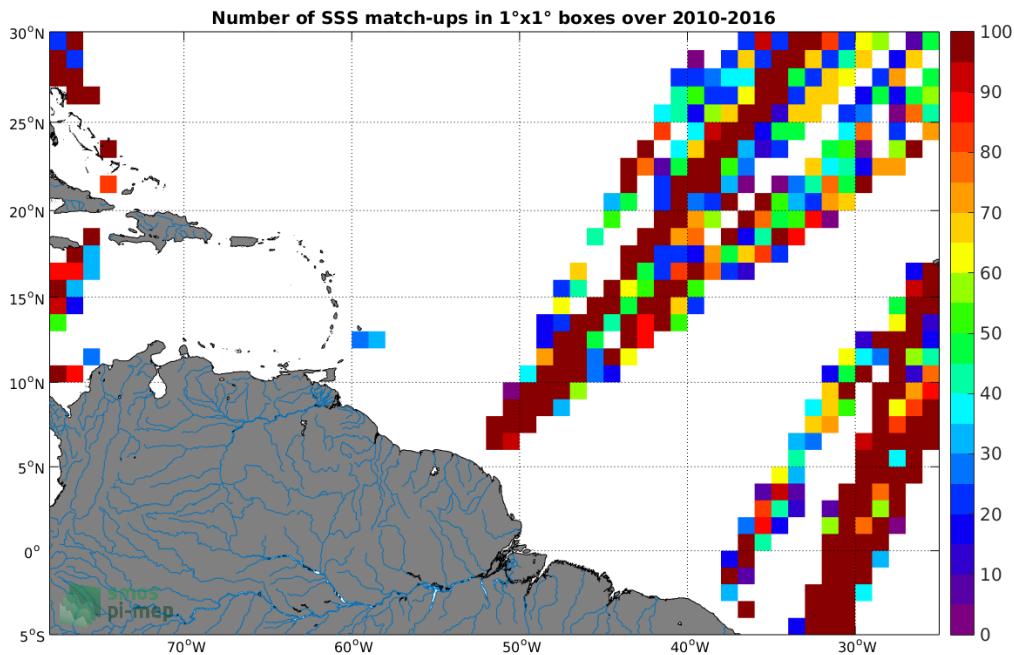
Figure 4: Number of SSS match-ups between TSG-LEGOS-DM SSS and the SMOS-L3-CATDS-CECOS-IFREMER-V2-1DAY-0.5DEG SSS product for the Amazon and Orinoco river plumes Pi-MEP region over 1^\circ \times 1^\circ boxes and for the full satellite product period.
