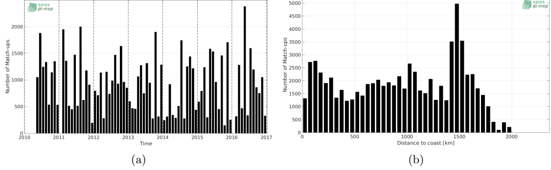
Figure 1: Number of match-ups between TSG-LEGOS-DM and SMOS-L3-CATDS-CECOS-IFREMER-V2-1DAY-0.5DEG SSS as a function of time (a) and as function of the distance to coast (b) over the Amazon and Orinoco river plumes Pi-MEP region and for the full satellite product period.
