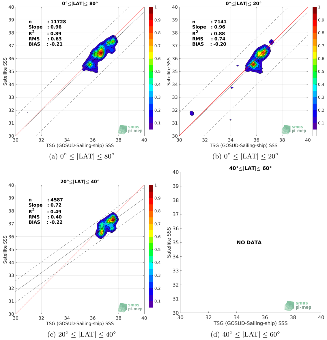
Figure 9: Contour maps of the concentration of SMOS SSS L3 v2 - Daily - 0.5 Deg (CATDS-CECOS-IFREMER) SSS (y-axis) versus TSG (GOSUD-Sailing-ship) SSS (x-axis) at match-up pairs for different latitude bands. For each plot, the red line shows x=y . The black thin and dashed lines indicate a linear fit through the data cloud and the \pm 95\% confidence levels, respectively. The number match-up pairs n , the slope and R^2 coefficient of the linear fit, the root mean square (RMS) and the mean bias between satellite and in situ data are indicated for each latitude band in each plots.
