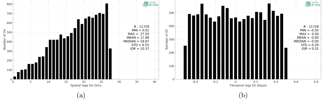
Figure 5: Histograms of the spatial (a) and temporal (b) lags between the location/time of the TSG (GOSUD-Sailing-ship) measurement and the date of the corresponding SMOS SSS L3 v2 - Daily - 0.5 Deg (CATDS-CECOS-IFREMER) SSS pixel.
