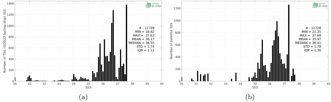
Figure 2: Histograms of SSS from TSG (GOSUD-Sailing-ship) (a) and SMOS SSS L3 v2 - Daily - 0.5 Deg (CATDS-CECOS-IFREMER) (b) considering all match-up pairs per bins of 0.1 over the Amazon and Orinoco river plumes Pi-MEP region and for the full satellite product period.
