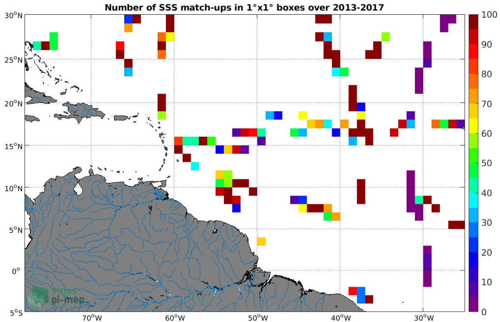
Figure 4: Number of SSS match-ups between TSG (GOSUD-Sailing-ship) SSS and the SMOS SSS L3 v2 - Daily - 0.5 Deg (CATDS-CECOS-IFREMER) SSS product for the Amazon and Orinoco river plumes Pi-MEP region over 1^\circ \times 1^\circ boxes and for the full satellite product period.
