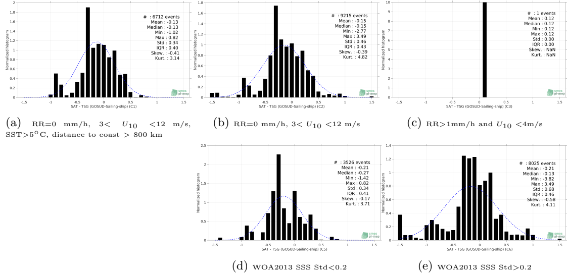
Figure 13: Normalized histogram of \Delta SSS (SMOS SSS L3 v2 - Daily - 0.5 Deg (CATDS-CECOS-IFREMER) - TSG (GOSUD-Sailing-ship)) for 5 different subdatasets corresponding to: RR=0 mm/h, 3 < U_{10} < 12 m/s, SST>5°C, distance to coast > 800 km (a), RR=0 mm/h, 3 < U_{10} < 12 m/s (b), RR>1mm/h and U_{10} < 4 m/s (c), WOA2013 SSS Std<0.2 (d), WOA2013 SSS Std>0.2 (e).
