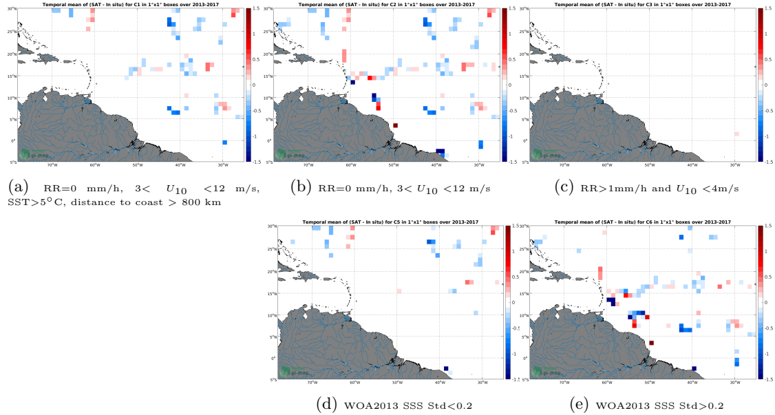
Figure 12: Temporal mean gridded over spatial boxes of size 1^\circ \times 1^\circ of \Delta SSS (SMOS SSS L3 v2 - Daily - 0.5 Deg (CATDS-CECOS-IFREMER) - TSG (GOSUD-Sailing-ship)) for 5 different subdatasets corresponding to: RR=0 mm/h, 3 < U_{10} < 12 m/s, SST >5^\circ\text{C} , distance to coast > 800 km (a), RR=0 mm/h, 3 < U_{10} < 12 m/s (b), RR >1 mm/h and U_{10} < 4 m/s (c), WOA2013 SSS Std <0.2 (d), WOA2013 SSS Std >0.2 (e).
