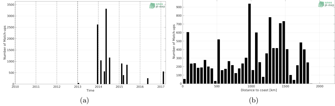
Figure 1: Number of match-ups between TSG (GOSUD-Sailing-ship) and SMOS SSS L3 v2 - Daily - 0.5 Deg (CATDS-CECOS-IFREMER) SSS as a function of time (a) and as function of the distance to coast (b) over the Amazon and Orinoco river plumes Pi-MEP region and for the full satellite product period.
