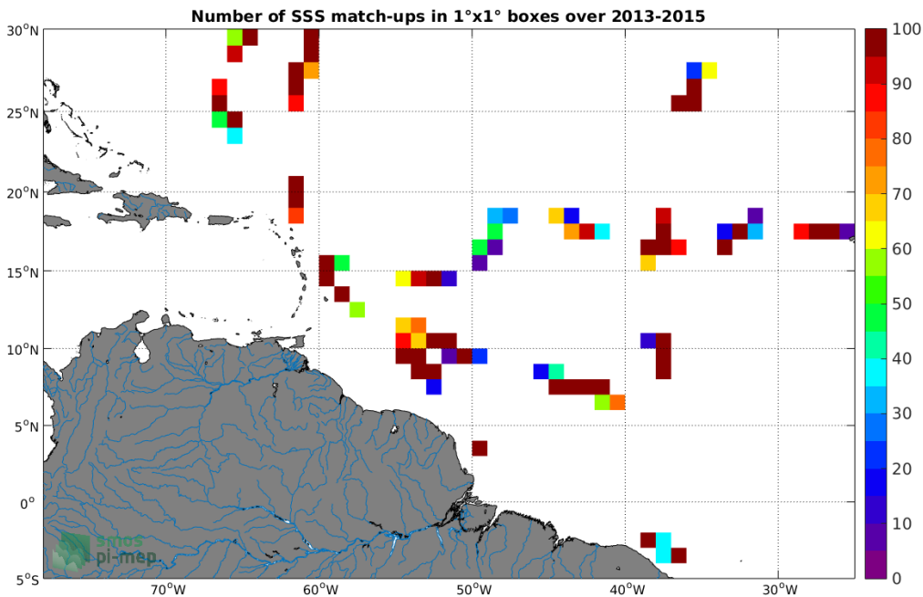
Figure 4: Number of SSS match-ups between TSG-GOSUD-Sailing-ship SSS and the SMOS-L3-CATDS-CECOS-IFREMER-V2-1DAY-0.5DEG SSS product for the Amazon and Orinoco river plumes Pi-MEP region over 1°x1° boxes and for the full satellite product period.
