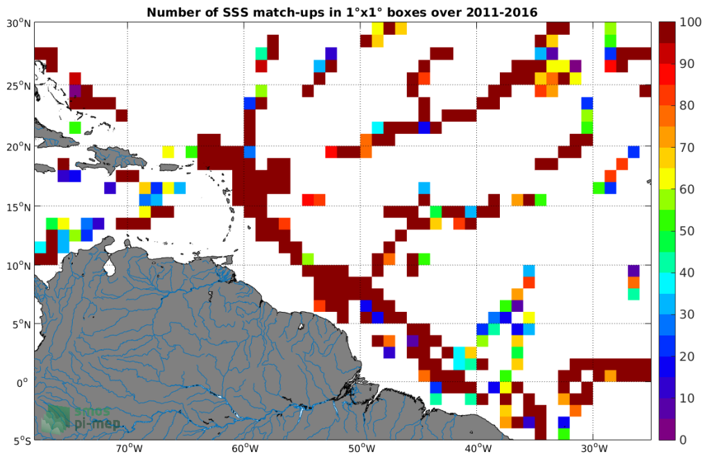
Figure 4: Number of SSS match-ups between TSG-GOSUD-Research-vessel SSS and the SMOS-L3-CATDS-CECOS-IFREMER-V2-1DAY-0.5DEG SSS product for the Amazon and Orinoco river plumes Pi-MEP region over 1°x1° boxes and for the full satellite product period.
