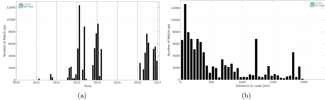
Figure 1: Number of match-ups between TSG-GOSUD-Research-vessel and SMOS-L3-CATDS-CECOS-IFREMER-V2-1DAY-0.5DEG SSS as a function of time (a) and as function of the distance to coast (b) over the Amazon and Orinoco river plumes Pi-MEP region and for the full satellite product period.
