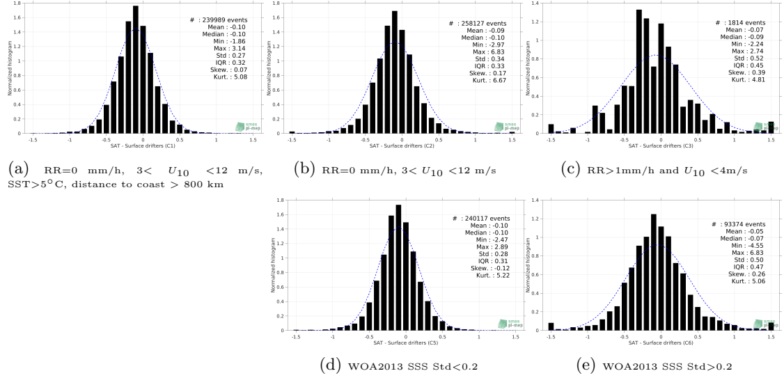
Figure 12: Normalized histogram of \Delta\text{SSS} (SMOS SSS L3 v2 - Daily - 0.5 Deg (CATDS-CECOS-IFREMER) - Surface drifters) for 5 different subdatasets corresponding to: RR=0 mm/h, 3 < U_{10} < 12 m/s, SST > 5^\circ\text{C} , distance to coast > 800 km (a), RR=0 mm/h, 3 < U_{10} < 12 m/s (b), RR > 1\text{mm/h} and U_{10} < 4\text{m/s} (c), WOA2013 SSS Std < 0.2 (d), WOA2013 SSS Std > 0.2 (e).
