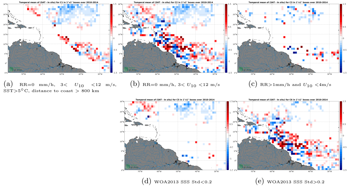
Figure 11: Temporal mean gridded over spatial boxes of size 1^{\circ}\times 1^{\circ} of \Delta\text{SSS} (SMOS SSS L3 v2 - Daily - 0.5 Deg (CATDS-CECOS-IFREMER) - Surface drifters) for 5 different subdatasets corresponding to:RR=0 mm/h, 3 < U_{10} < 12 m/s, SST >5^{\circ}\text{C} , distance to coast > 800 km (a), RR=0 mm/h, 3 < U_{10} < 12 m/s (b), RR >1 mm/h and U_{10} < 4 m/s (c), WOA2013 SSS Std <0.2 (d), WOA2013 SSS Std >0.2 (e).
