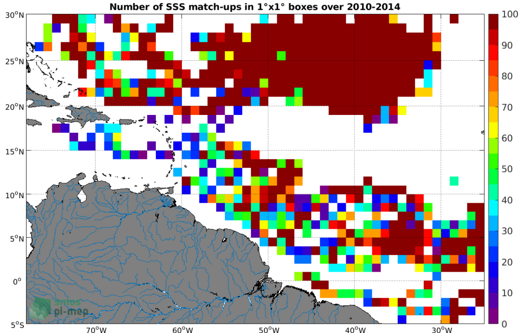
Figure 3: Number of SSS match-ups between Surface drifters SSS and the SMOS SSS L3 v2 - Daily - 0.5 Deg (CATDS-CECOS-IFREMER) SSS product for the Amazon and Orinoco river plumes Pi-MEP region over 1^\circ \times 1^\circ boxes and for the full satellite product period.
