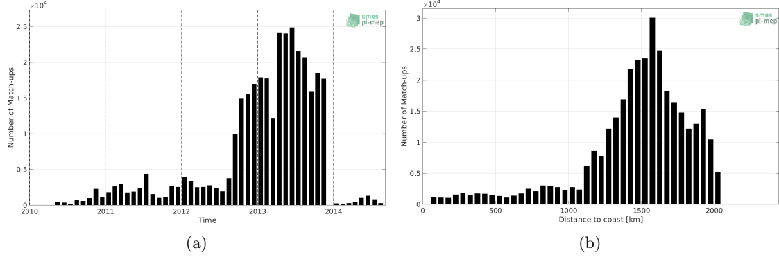
Figure 1: Number of match-ups between Surface drifters and SMOS SSS L3 v2 - Daily - 0.5 Deg (CATDS-CECOS-IFREMER) SSS as a function of time (a) and as function of the distance to coast (b) over the Amazon and Orinoco river plumes Pi-MEP region and for the full satellite product period.
