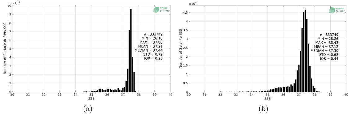
Figure 2: Histograms of SSS from Surface drifters (a) and SMOS SSS L3 v2 - Daily - 0.5 Deg (CATDS-CECOS-IFREMER) (b) considering all match-up pairs per bins of 0.1 over the Amazon and Orinoco river plumes Pi-MEP region and for the full satellite product period.
