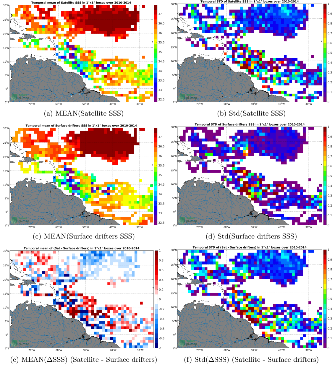
Figure 5: Temporal mean (left) and Std (right) of SSS from SMOS SSS L3 v2 - Daily - 0.5 Deg (CATDS-CECOS-IFREMER) (top), Surface drifters (middle), and of \Delta SSS (Satellite - Surface drifters). Only match-up pairs are used to generate these maps.
