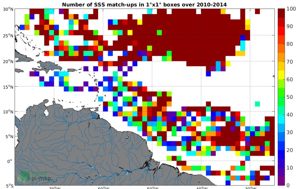
Figure 3: Number of SSS match-ups between Surface drifters SSS and the SMOS-L3-CATDS-CECOS-IFREMER-V2-1DAY-0.5DEG SSS product for the Amazon and Orinoco river plumes Pi-MEP region over 1^\circ \times 1^\circ boxes and for the full satellite product period.
