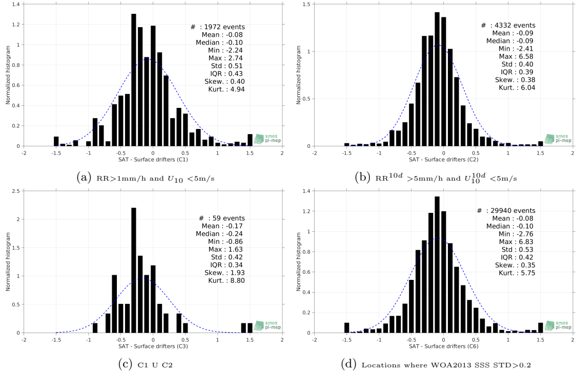
Figure 12: Normalized histogram of \Delta SSS (SMOS-L3-CATDS-CECOS-IFREMER-V2-1DAY-0.5DEG - Surface drifters) for 6 different subdatasets corresponding to: RR > 1mm/h and U_{10} < 5\text{m/s} (a), RR^{10d} > 5\text{mm/h} and U_{10}^{10d} < 5\text{m/s} (b), C1 U C2 (c), Locations where WOA2013 SSS STD > 0.2 (d).
