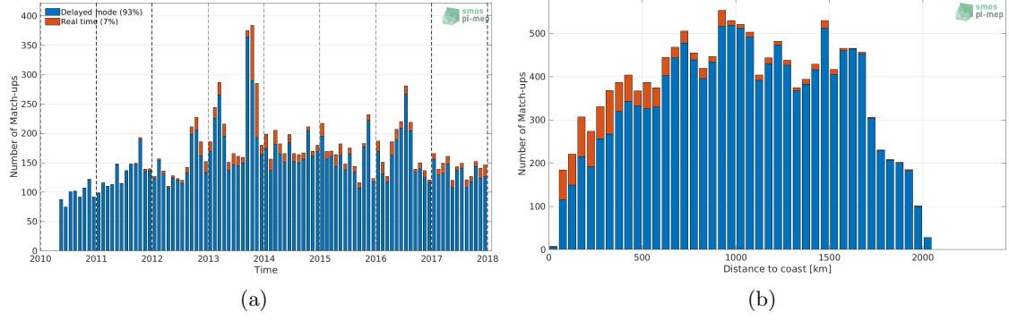
Figure 1: Number of match-ups between Argo and SMOS SSS L3 v2 - Daily - 0.5 Deg (CATDS-CECOS-IFREMER) SSS as a function of time (a) and as function of the distance to coast (b) over the Amazon and Orinoco river plumes Pi-MEP region and for the full satellite product period.
