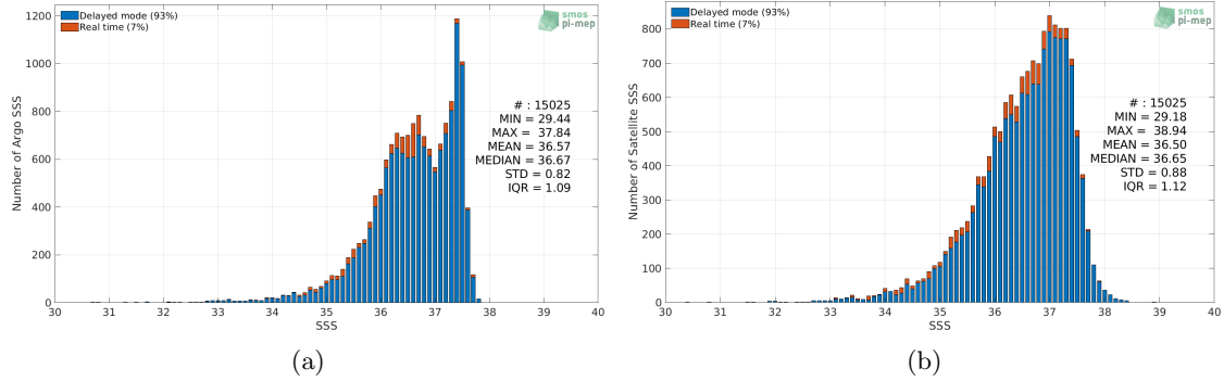
Figure 2: Histograms of SSS from Argo (a) and SMOS SSS L3 v2 - Daily - 0.5 Deg (CATDS-CECOS-IFREMER) (b) considering all match-up pairs per bins of 0.1 over the Amazon and Orinoco river plumes Pi-MEP region and for the full satellite product period.
