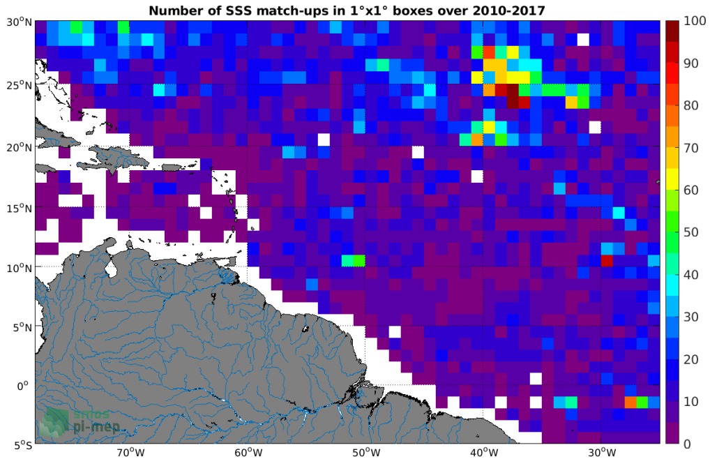
Figure 4: Number of SSS match-ups between Argo SSS and the SMOS SSS L3 v2 - Daily - 0.5 Deg (CATDS-CECOS-IFREMER) SSS product for the Amazon and Orinoco river plumes Pi-MEP region over 1^\circ \times 1^\circ boxes and for the full satellite product period.
