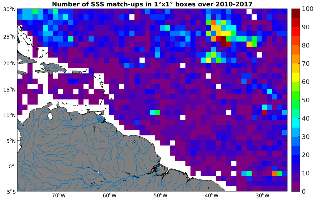
Figure 4: Number of SSS match-ups between Argo SSS and the SMOS-L3-CATDS-CECOS-IFREMER-V2-1DAY-0.5DEG SSS product for the Amazon and Orinoco river plumes Pi-MEP region over 1^\circ \times 1^\circ boxes and for the full satellite product period.
