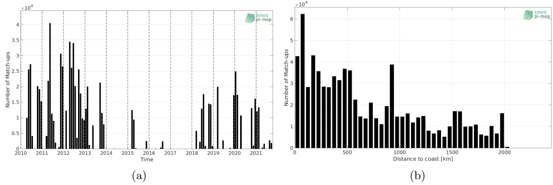
Figure 1: Number of match-ups between TSG (SAMOS) and SMOS SSS L3 v335 - Monthly - 25 km (CATDS-CPDC) SSS as a function of time (a) and as function of the distance to coast (b) over the Amazon and Orinoco river plumes Pi-MEP region and for the full satellite product period.
