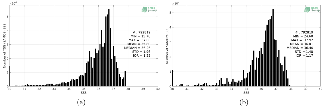
Figure 2: Histograms of SSS from TSG (SAMOS) (a) and SMOS SSS L3 v335 - Monthly - 25 km (CATDS-CPDC) (b) considering all match-up pairs per bins of 0.1 over the Amazon and Orinoco river plumes Pi-MEP region and for the full satellite product period.
