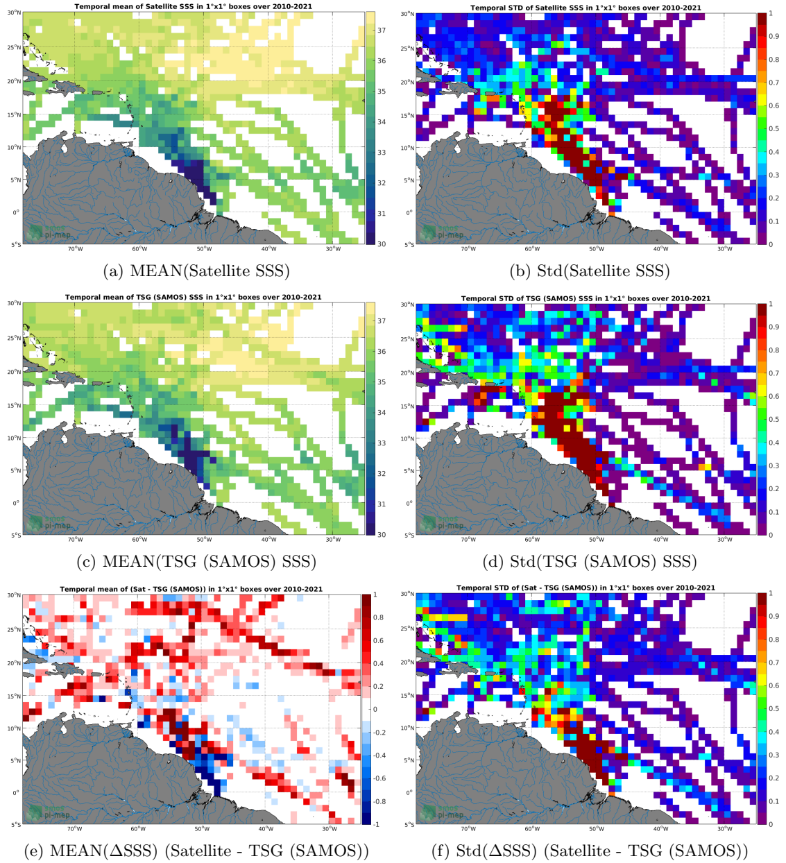
Figure 6: Temporal mean (left) and Std (right) of SSS from SMOS SSS L3 v335 - Monthly - 25 km (CATDS-CPDC) (top), TSG (SAMOS) (middle), and of \Delta SSS (Satellite - TSG (SAMOS)). Only match-up pairs are used to generate these maps.
