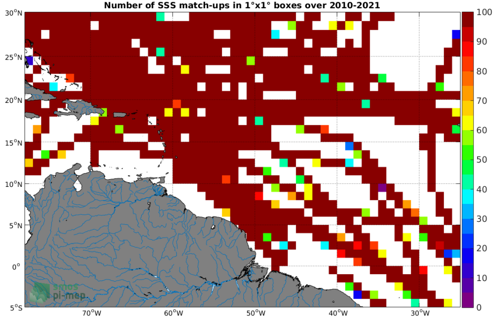
Figure 4: Number of SSS match-ups between TSG (SAMOS) SSS and the SMOS SSS L3 v335 - Monthly - 25 km (CATDS-CPDC) SSS product for the Amazon and Orinoco river plumes Pi-MEP region over 1^\circ \times 1^\circ boxes and for the full satellite product period.
