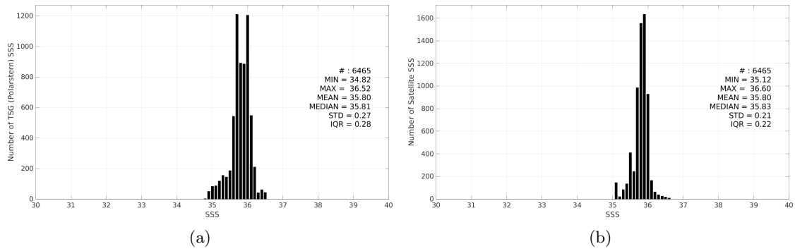
Figure 3: Histograms of SSS from TSG (Polarstern) (a) and SMOS SSS L3 v335 - Monthly - 25 km (CATDS-CPDC) (b) considering all match-up pairs per bins of 0.1 over the Amazon and Orinoco river plumes Pi-MEP region and for the full satellite product period.
