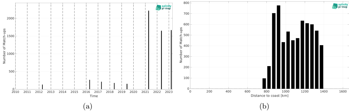
Figure 2: Number of match-ups between TSG (Polarstern) and SMOS SSS L3 v335 - Monthly - 25 km (CATDS-CPDC) SSS as a function of time (a) and as function of the distance to coast (b) over the Amazon and Orinoco river plumes Pi-MEP region and for the full satellite product period.
