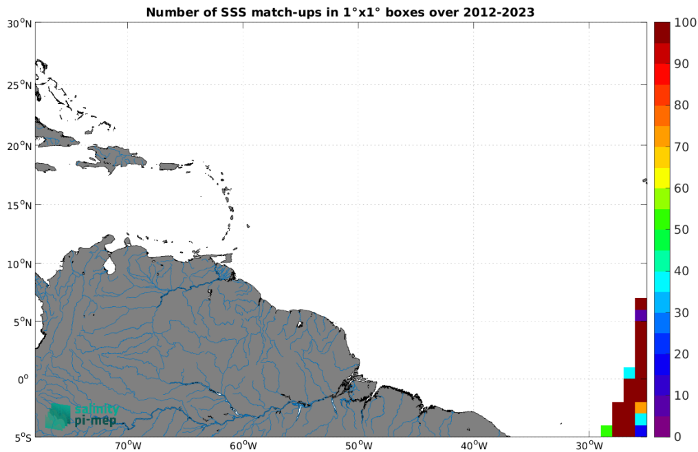
Figure 5: Number of SSS match-ups between TSG (Polarstern) SSS and the SMOS SSS L3 v335 - Monthly - 25 km (CATDS-CPDC) SSS product for the Amazon and Orinoco river plumes Pi-MEP region over 1^\circ \times 1^\circ boxes and for the full satellite product period.
