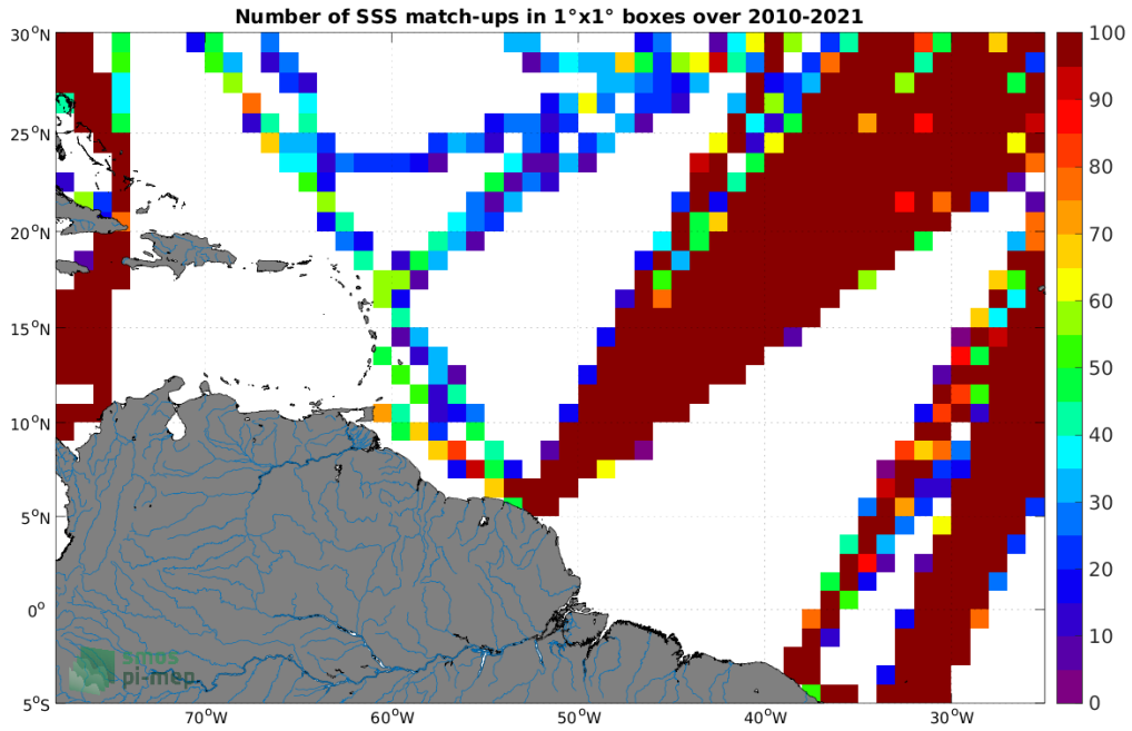
Figure 4: Number of SSS match-ups between TSG (LEGOS-DM) SSS and the SMOS SSS L3 v335 - Monthly - 25 km (CATDS-CPDC) SSS product for the Amazon and Orinoco river plumes Pi-MEP region over 1^{\circ} \times 1^{\circ} boxes and for the full satellite product period.
