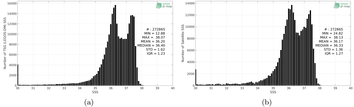
Figure 2: Histograms of SSS from TSG (LEGOS-DM) (a) and SMOS SSS L3 v335 - Monthly - 25 km (CATDS-CPDC) (b) considering all match-up pairs per bins of 0.1 over the Amazon and Orinoco river plumes Pi-MEP region and for the full satellite product period.
