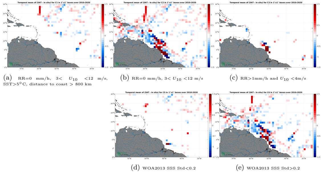
Figure 12: Temporal mean gridded over spatial boxes of size 1^{\circ}\times 1^{\circ} of \Delta SSS (SMOS SSS L3 v335 - Monthly - 25 km (CATDS-CPDC) - TSG (GOSUD-Research-vessel)) for 5 different subdatasets corresponding to:RR=0 mm/h, 3 < U_{10} < 12 m/s, SST >5^{\circ}\text{C} , distance to coast > 800 km (a), RR=0 mm/h, 3 < U_{10} < 12 m/s (b), RR >1 mm/h and U_{10} < 4 m/s (c), WOA2013 SSS Std <0.2 (d), WOA2013 SSS Std >0.2 (e).
