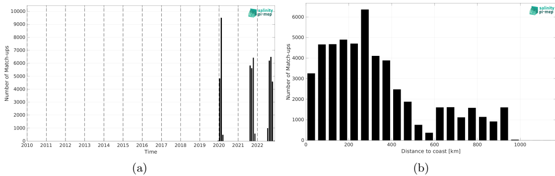
Figure 2: Number of match-ups between Saildrone and SMOS SSS L3 v335 - Monthly - 25 km (CATDS-CPDC) SSS as a function of time (a) and as function of the distance to coast (b) over the Amazon and Orinoco river plumes Pi-MEP region and for the full satellite product period.
