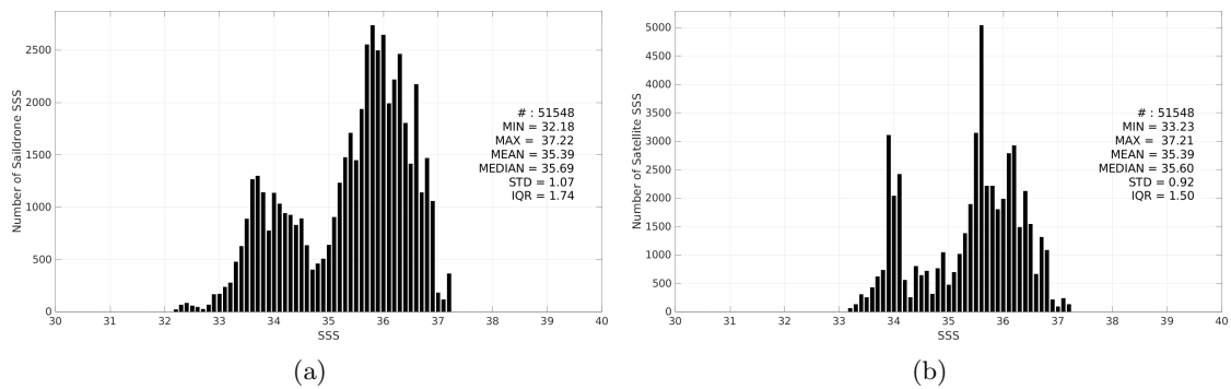
Figure 3: Histograms of SSS from Saildrone (a) and SMOS SSS L3 v335 - Monthly - 25 km (CATDS-CPDC) (b) considering all match-up pairs per bins of 0.1 over the Amazon and Orinoco river plumes Pi-MEP region and for the full satellite product period.
