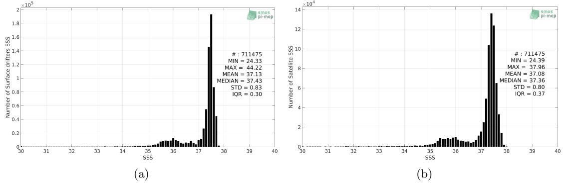
Figure 2: Histograms of SSS from Surface drifters (a) and SMOS SSS L3 v335 - Monthly - 25 km (CATDS-CPDC) (b) considering all match-up pairs per bins of 0.1 over the Amazon and Orinoco river plumes Pi-MEP region and for the full satellite product period.
