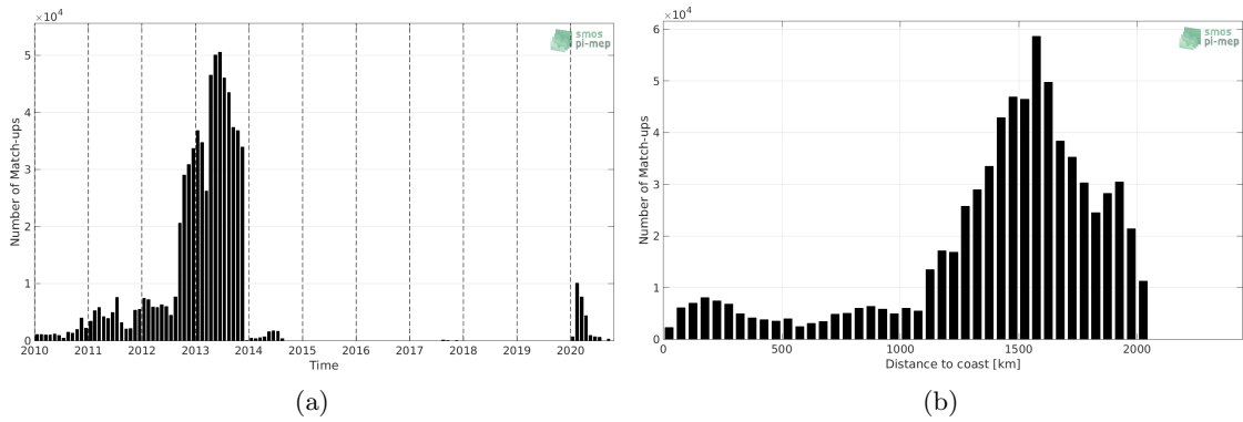
Figure 1: Number of match-ups between Surface drifters and SMOS SSS L3 v335 - Monthly - 25 km (CATDS-CPDC) SSS as a function of time (a) and as function of the distance to coast (b) over the Amazon and Orinoco river plumes Pi-MEP region and for the full satellite product period.
