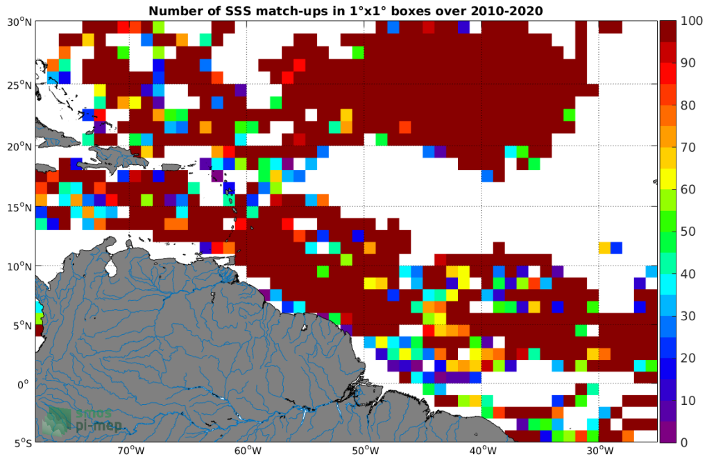
Figure 3: Number of SSS match-ups between Surface drifters SSS and the SMOS SSS L3 v335 - Monthly - 25 km (CATDS-CPDC) SSS product for the Amazon and Orinoco river plumes Pi-MEP region over 1^\circ \times 1^\circ boxes and for the full satellite product period.
