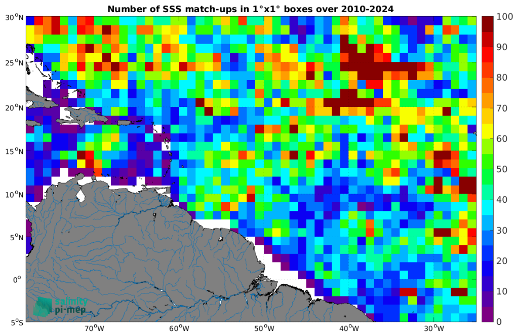
Figure 5: Number of SSS match-ups between Argo SSS and the SMOS SSS L3 v335 - Monthly - 25 km (CATDS-CPDC) SSS product for the Amazon and Orinoco river plumes Pi-MEP region over 1^{\circ} \times 1^{\circ} boxes and for the full satellite product period.
