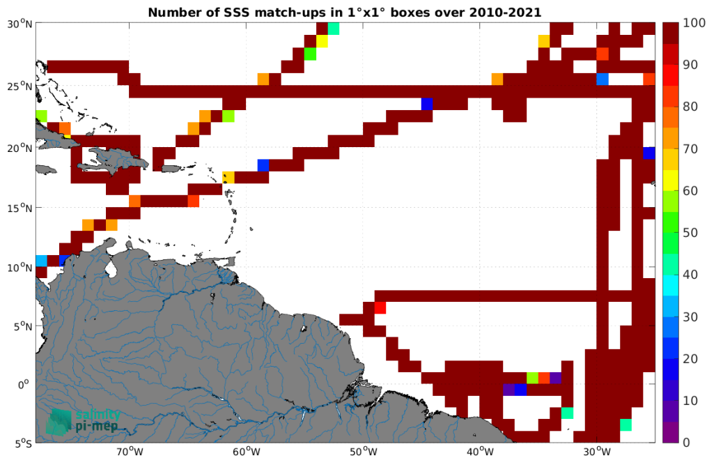
Figure 5: Number of SSS match-ups between TSG (CSIC-UTM) SSS and the SMOS SSS L3 v335 - 10 Days - 25 km (CATDS-CPDC) SSS product for the Amazon and Orinoco river plumes Pi-MEP region over 1^\circ \times 1^\circ boxes and for the full satellite product period.
