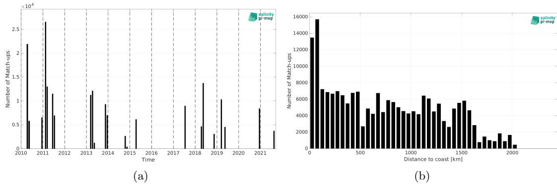
Figure 2: Number of match-ups between TSG (CSIC-UTM) and SMOS SSS L3 v335 - 10 Days - 25 km (CATDS-CPDC) SSS as a function of time (a) and as function of the distance to coast (b) over the Amazon and Orinoco river plumes Pi-MEP region and for the full satellite product period.
