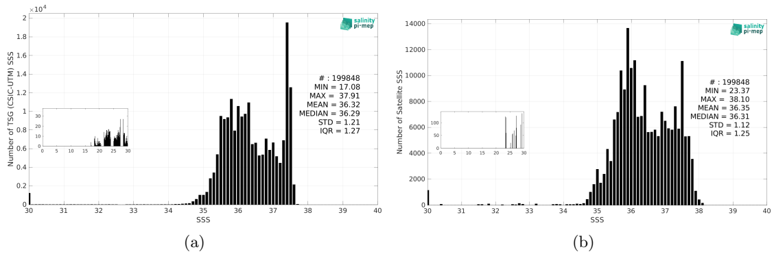
Figure 3: Histograms of SSS from TSG (CSIC-UTM) (a) and SMOS SSS L3 v335 - 10 Days - 25 km (CATDS-CPDC) (b) considering all match-up pairs per bins of 0.1 over the Amazon and Orinoco river plumes Pi-MEP region and for the full satellite product period.
