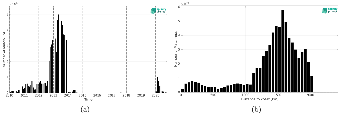
Figure 2: Number of match-ups between Surface drifters and SMOS SSS L3 v335 - 10 Days - 25 km (CATDS-CPDC) SSS as a function of time (a) and as function of the distance to coast (b) over the Amazon and Orinoco river plumes Pi-MEP region and for the full satellite product period.
