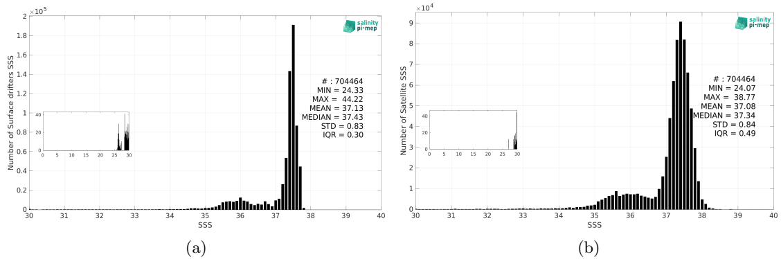
Figure 3: Histograms of SSS from Surface drifters (a) and SMOS SSS L3 v335 - 10 Days - 25 km (CATDS-CPDC) (b) considering all match-up pairs per bins of 0.1 over the Amazon and Orinoco river plumes Pi-MEP region and for the full satellite product period.
