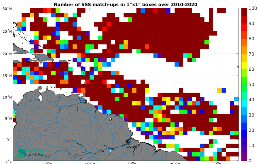
Figure 4: Number of SSS match-ups between Surface drifters SSS and the SMOS SSS L3 v335 - 10 Days - 25 km (CATDS-CPDC) SSS product for the Amazon and Orinoco river plumes Pi-MEP region over 1^\circ \times 1^\circ boxes and for the full satellite product period.
