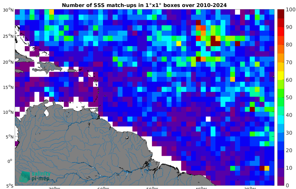
Figure 5: Number of SSS match-ups between Argo SSS and the SMOS SSS L2Q v333 - 0.25 Deg (CATDS-CPDC) SSS product for the Amazon and Orinoco river plumes Pi-MEP region over 1^\circ \times 1^\circ boxes and for the full satellite product period.
