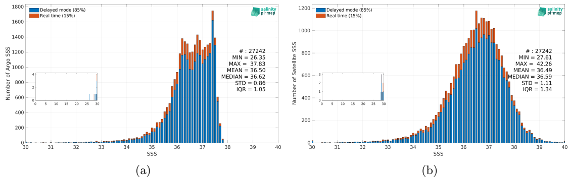
Figure 3: Histograms of SSS from Argo (a) and SMOS SSS L2Q v333 - 0.25 Deg (CATDS-CPDC) (b) considering all match-up pairs per bins of 0.1 over the Amazon and Orinoco river plumes Pi-MEP region and for the full satellite product period.
