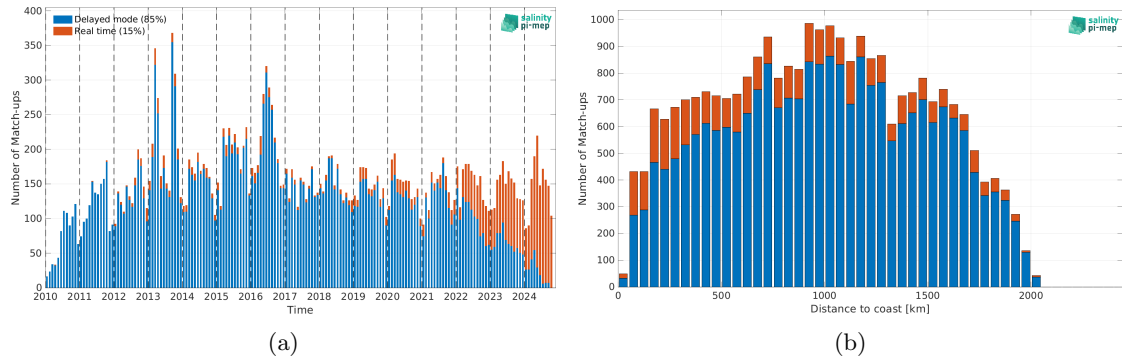
Figure 2: Number of match-ups between Argo and SMOS SSS L2Q v333 - 0.25 Deg (CATDS-CPDC) SSS as a function of time (a) and as function of the distance to coast (b) over the Amazon and Orinoco river plumes Pi-MEP region and for the full satellite product period.
