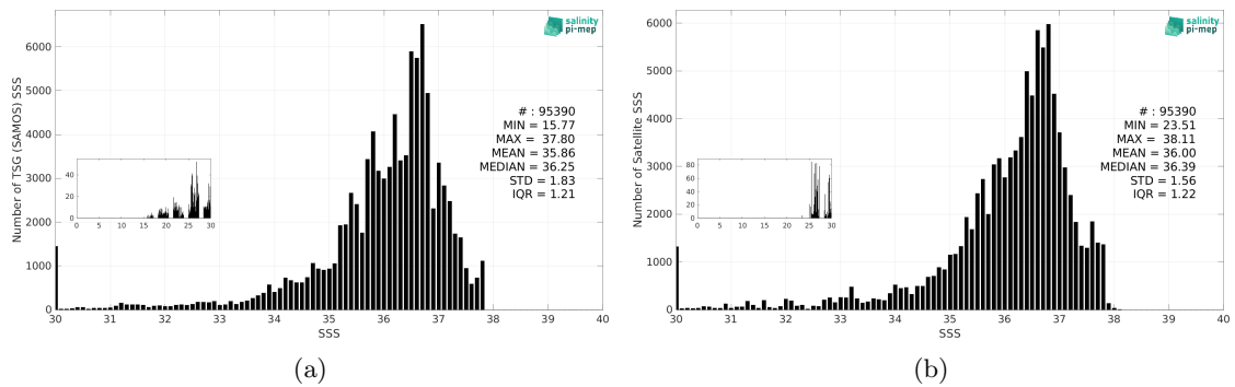
Figure 3: Histograms of SSS from TSG (SAMOS) (a) and SMOS SSS L3 v332 - 9 Days (CATDS-CPDC) (b) considering all match-up pairs per bins of 0.1 over the Amazon and Orinoco river plumes Pi-MEP region and for the full satellite product period.
