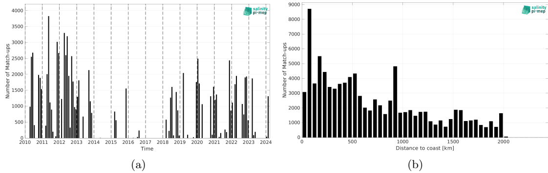
Figure 2: Number of match-ups between TSG (SAMOS) and SMOS SSS L3 v332 - 9 Days (CATDS-CPDC) SSS as a function of time (a) and as function of the distance to coast (b) over the Amazon and Orinoco river plumes Pi-MEP region and for the full satellite product period.
