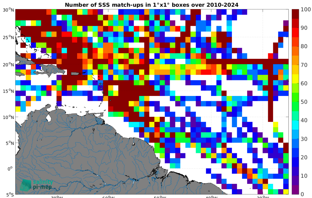
Figure 5: Number of SSS match-ups between TSG (SAMOS) SSS and the SMOS SSS L3 v332 - 9 Days (CATDS-CPDC) SSS product for the Amazon and Orinoco river plumes Pi-MEP region over 1^\circ \times 1^\circ boxes and for the full satellite product period.
