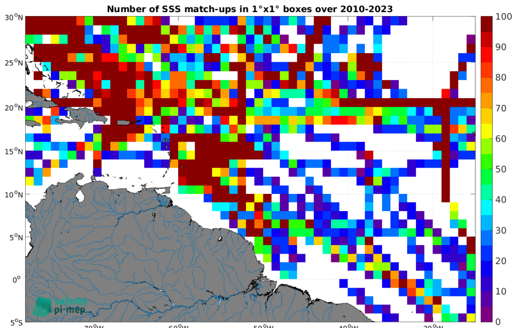
Figure 4: Number of SSS match-ups between TSG (SAMOS) SSS and the SMOS SSS L3 v332 - 9 Days (CATDS-CPDC) SSS product for the Amazon and Orinoco river plumes Pi-MEP region over 1^\circ \times 1^\circ boxes and for the full satellite product period.
