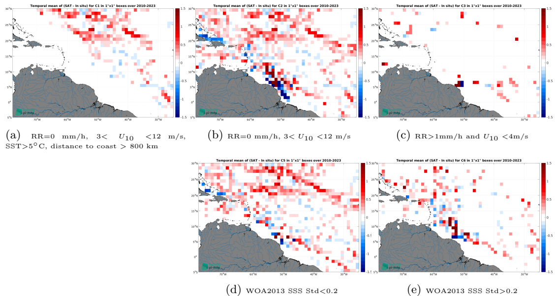
Figure 12: Temporal mean gridded over spatial boxes of size 1^\circ \times 1^\circ of \Delta SSS (SMOS SSS L3 v332 - 9 Days (CATDS-CPDC) - TSG (SAMOS)) for 5 different subdatasets corresponding to:RR=0 mm/h, 3 < U_{10} < 12 m/s, SST > 5^\circ\text{C} , distance to coast > 800 km (a), RR=0 mm/h, 3 < U_{10} < 12 m/s (b), RR > 1 mm/h and U_{10} < 4 m/s (c), WOA2013 SSS Std < 0.2 (d), WOA2013 SSS Std > 0.2 (e).
