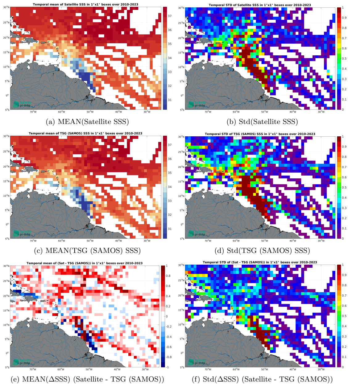
Figure 6: Temporal mean (left) and Std (right) of SSS from SMOS SSS L3 v332 - 9 Days (CATDS-CPDC) (top), TSG (SAMOS) (middle), and of \Delta SSS (Satellite - TSG (SAMOS)). Only match-up pairs are used to generate these maps.
