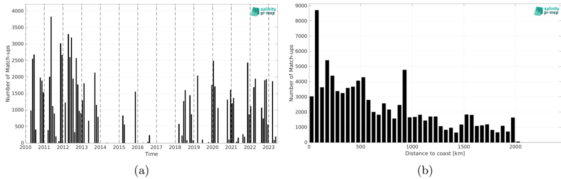
Figure 1: Number of match-ups between TSG (SAMOS) and SMOS SSS L3 v332 - 9 Days (CATDS-CPDC) SSS as a function of time (a) and as function of the distance to coast (b) over the Amazon and Orinoco river plumes Pi-MEP region and for the full satellite product period.
