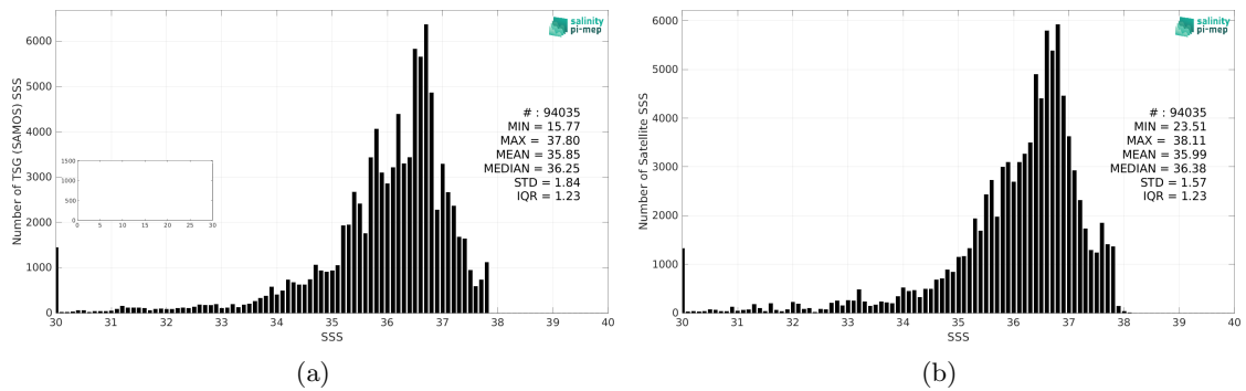
Figure 2: Histograms of SSS from TSG (SAMOS) (a) and SMOS SSS L3 v332 - 9 Days (CATDS-CPDC) (b) considering all match-up pairs per bins of 0.1 over the Amazon and Orinoco river plumes Pi-MEP region and for the full satellite product period.
