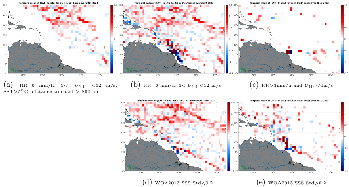
Figure 12: Temporal mean gridded over spatial boxes of size 1^\circ \times 1^\circ of \Delta SSS (SMOS SSS L3 v332 - 9 Days (CATDS-CPDC) - TSG (SAMOS)) for 5 different subdatasets corresponding to:RR=0 mm/h, 3 < U_{10} < 12 m/s, SST >5^\circ\text{C} , distance to coast > 800 km (a), RR=0 mm/h, 3 < U_{10} < 12 m/s (b), RR >1 mm/h and U_{10} < 4 m/s (c), WOA2013 SSS Std <0.2 (d), WOA2013 SSS Std >0.2 (e).
