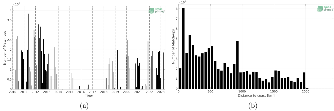
Figure 1: Number of match-ups between TSG (SAMOS) and SMOS SSS L3 v332 - 9 Days (CATDS-CPDC) SSS as a function of time (a) and as function of the distance to coast (b) over the Amazon and Orinoco river plumes Pi-MEP region and for the full satellite product period.
