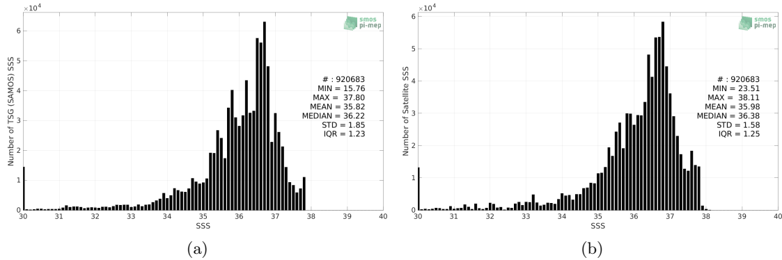
Figure 2: Histograms of SSS from TSG (SAMOS) (a) and SMOS SSS L3 v332 - 9 Days (CATDS-CPDC) (b) considering all match-up pairs per bins of 0.1 over the Amazon and Orinoco river plumes Pi-MEP region and for the full satellite product period.
