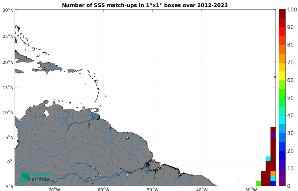
Figure 5: Number of SSS match-ups between TSG (Polarstern) SSS and the SMOS SSS L3 v332 - 9 Days (CATDS-CPDC) SSS product for the Amazon and Orinoco river plumes Pi-MEP region over 1^\circ \times 1^\circ boxes and for the full satellite product period.
