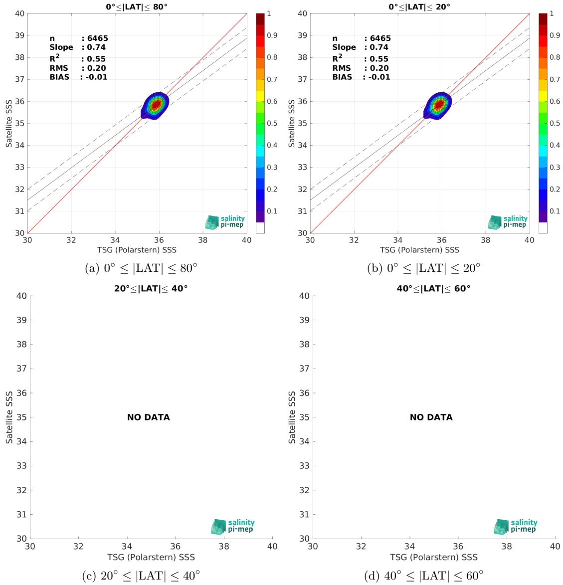
Figure 10: Contour maps of the concentration of SMOS SSS L3 v332 - 9 Days (CATDS-CPDC) SSS (y-axis) versus TSG (Polarstern) SSS (x-axis) at match-up pairs for different latitude bands. For each plot, the red line shows x=y . The black thin and dashed lines indicate a linear fit through the data cloud and the \pm 95\% confidence levels, respectively. The number match-up pairs n , the slope and R^2 coefficient of the linear fit, the root mean square (RMS) and the mean bias between satellite and in situ data are indicated for each latitude band in each plots.
