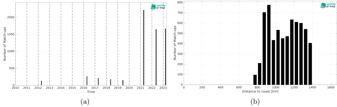
Figure 2: Number of match-ups between TSG (Polarstern) and SMOS SSS L3 v332 - 9 Days (CATDS-CPDC) SSS as a function of time (a) and as function of the distance to coast (b) over the Amazon and Orinoco river plumes Pi-MEP region and for the full satellite product period.
