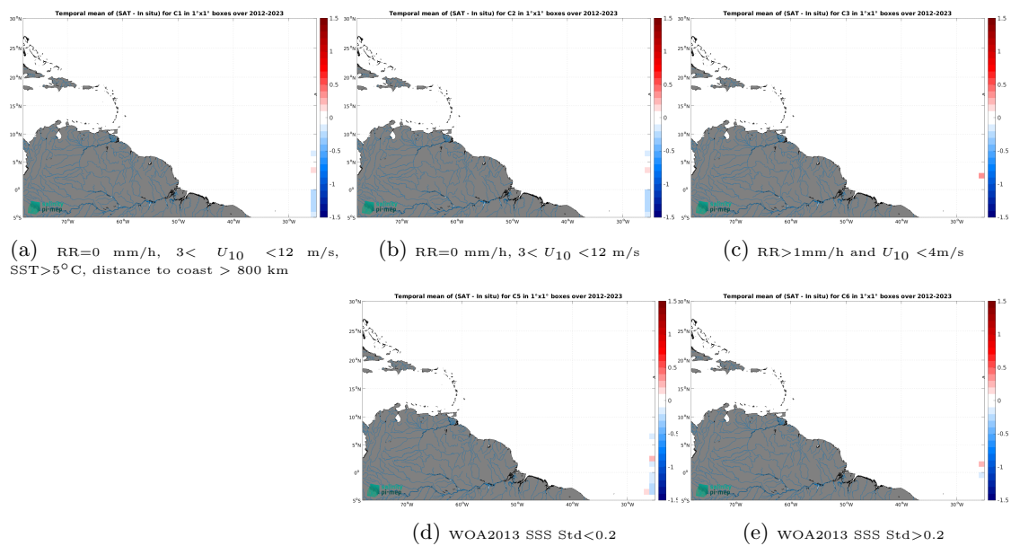
Figure 14: Temporal mean gridded over spatial boxes of size 1^\circ \times 1^\circ of \Delta SSS (SMOS SSS L3 v332 - 9 Days (CATDS-CPDC) - TSG (Polarstern)) for 5 different subdatasets corresponding to:RR=0 mm/h, 3 < U_{10} < 12 m/s, SST >5^\circ\text{C} , distance to coast > 800 km (a), RR=0 mm/h, 3 < U_{10} < 12 m/s (b), RR >1 mm/h and U_{10} < 4 m/s (c), WOA2013 SSS Std <0.2 (d), WOA2013 SSS Std >0.2 (e).
