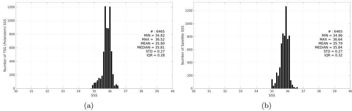
Figure 3: Histograms of SSS from TSG (Polarstern) (a) and SMOS SSS L3 v332 - 9 Days (CATDS-CPDC) (b) considering all match-up pairs per bins of 0.1 over the Amazon and Orinoco river plumes Pi-MEP region and for the full satellite product period.
