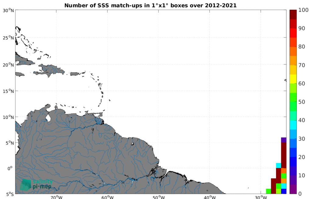
Figure 4: Number of SSS match-ups between TSG (Polarstern) SSS and the SMOS SSS L3 v332 - 9 Days (CATDS-CPDC) SSS product for the Amazon and Orinoco river plumes Pi-MEP region over 1^\circ \times 1^\circ boxes and for the full satellite product period.
