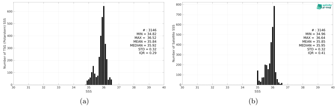
Figure 2: Histograms of SSS from TSG (Polarstern) (a) and SMOS SSS L3 v332 - 9 Days (CATDS-CPDC) (b) considering all match-up pairs per bins of 0.1 over the Amazon and Orinoco river plumes Pi-MEP region and for the full satellite product period.
