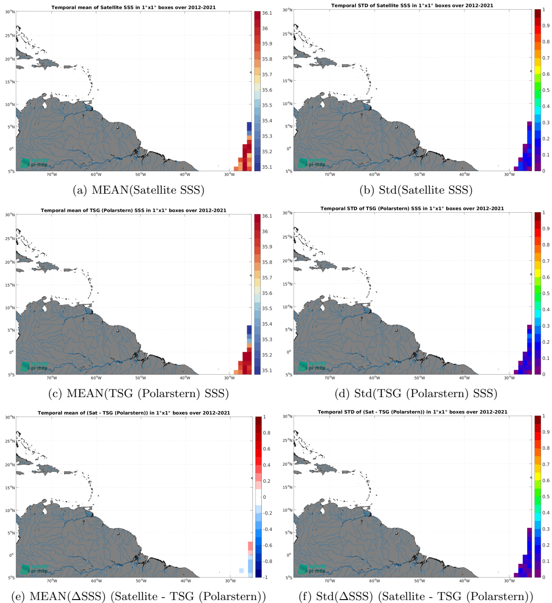
Figure 6: Temporal mean (left) and Std (right) of SSS from SMOS SSS L3 v332 - 9 Days (CATDS-CPDC) (top), TSG (Polarstern) (middle), and of \Delta SSS (Satellite - TSG (Polarstern)). Only match-up pairs are used to generate these maps.
