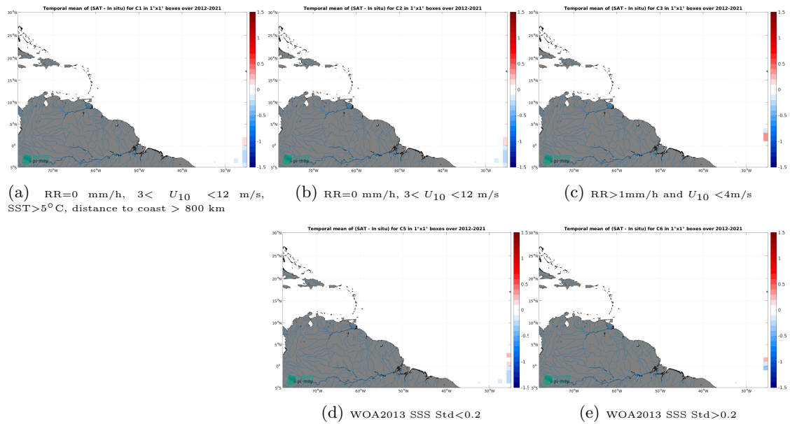
Figure 12: Temporal mean gridded over spatial boxes of size 1^\circ \times 1^\circ of \Delta SSS (SMOS SSS L3 v332 - 9 Days (CATDS-CPDC) - TSG (Polarstern)) for 5 different subdatasets corresponding to:RR=0 mm/h, 3 < U_{10} < 12 m/s, SST >5^\circ C, distance to coast > 800 km (a), RR=0 mm/h, 3 < U_{10} < 12 m/s (b), RR >1 mm/h and U_{10} < 4 m/s (c), WOA2013 SSS Std <0.2 (d), WOA2013 SSS Std >0.2 (e).
