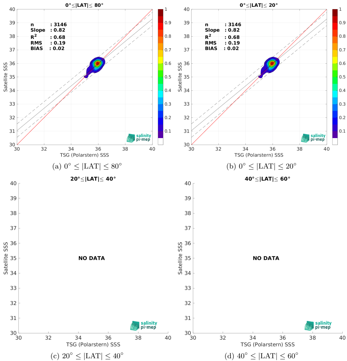
Figure 9: Contour maps of the concentration of SMOS SSS L3 v332 - 9 Days (CATDS-CPDC) SSS (y-axis) versus TSG (Polarstern) SSS (x-axis) at match-up pairs for different latitude bands. For each plot, the red line shows x=y . The black thin and dashed lines indicate a linear fit through the data cloud and the \pm 95\% confidence levels, respectively. The number match-up pairs n , the slope and R^2 coefficient of the linear fit, the root mean square (RMS) and the mean bias between satellite and in situ data are indicated for each latitude band in each plots.
