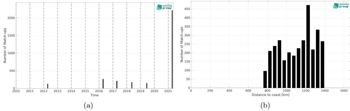
Figure 1: Number of match-ups between TSG (Polarstern) and SMOS SSS L3 v332 - 9 Days (CATDS-CPDC) SSS as a function of time (a) and as function of the distance to coast (b) over the Amazon and Orinoco river plumes Pi-MEP region and for the full satellite product period.
