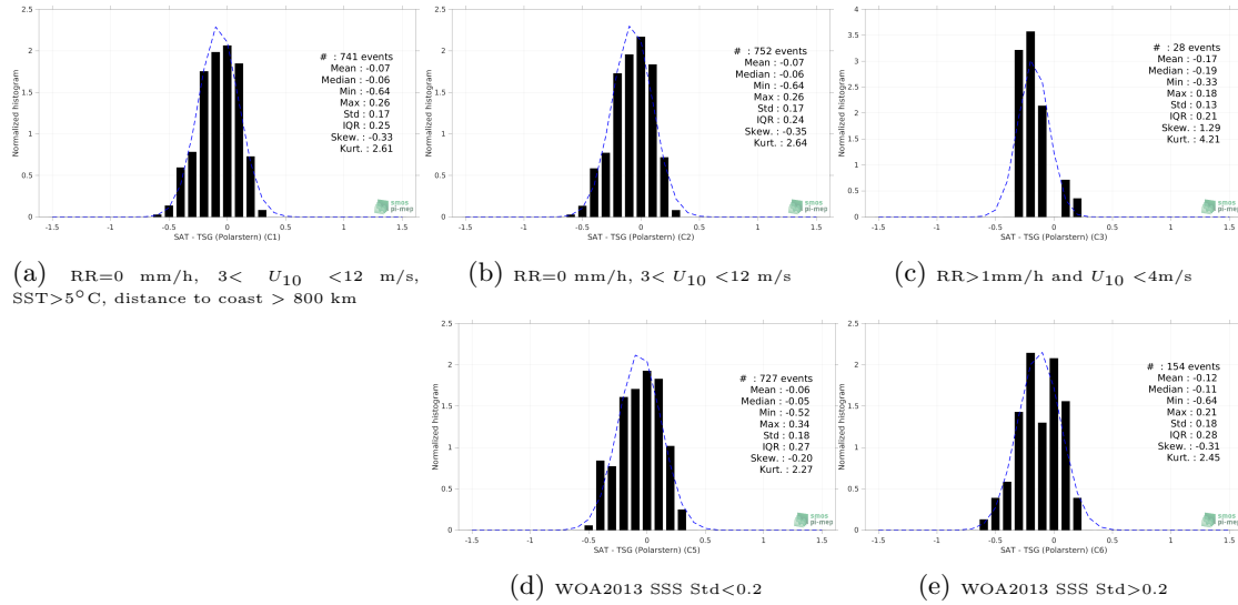
Figure 13: Normalized histogram of \Delta SSS (SMOS SSS L3 v332 - 9 Days (CATDS-CPDC) - TSG (Polarstern)) for 5 different subdatasets corresponding to: RR=0 mm/h, 3 < U_{10} < 12 m/s, SST > 5°C, distance to coast > 800 km (a), RR=0 mm/h, 3 < U_{10} < 12 m/s (b), RR > 1mm/h and U_{10} < 4 m/s (c), WOA2013 SSS Std < 0.2 (d), WOA2013 SSS Std > 0.2 (e).
