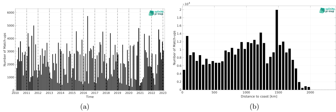
Figure 2: Number of match-ups between TSG (LEGOS-DM) and SMOS SSS L3 v332 - 9 Days (CATDS-CPDC) SSS as a function of time (a) and as function of the distance to coast (b) over the Amazon and Orinoco river plumes Pi-MEP region and for the full satellite product period.
