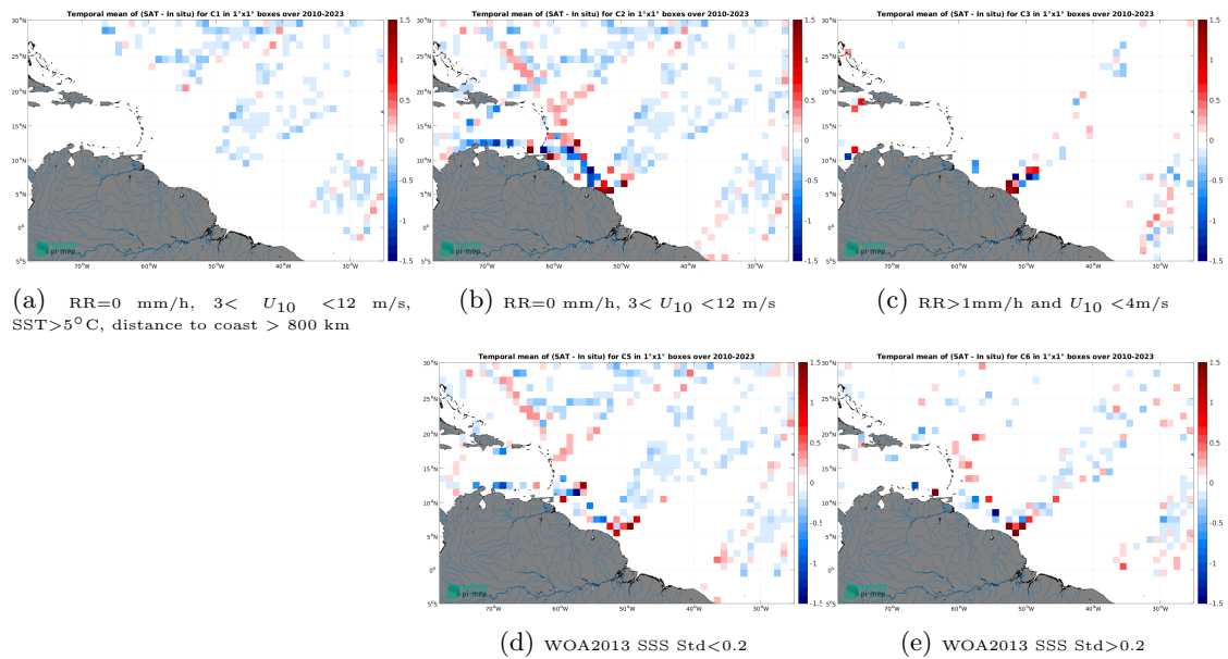
Figure 14: Temporal mean gridded over spatial boxes of size 1^\circ \times 1^\circ of \Delta\text{SSS} (SMOS SSS L3 v332 - 9 Days (CATDS-CPDC) - TSG (LEGOS-DM)) for 5 different subdatasets corresponding to:RR=0 mm/h, 3 < U_{10} < 12 m/s, SST >5^\circ\text{C} , distance to coast > 800 km (a), RR=0 mm/h, 3 < U_{10} < 12 m/s (b), RR >1 mm/h and U_{10} < 4 m/s (c), WOA2013 SSS Std <0.2 (d), WOA2013 SSS Std >0.2 (e).
