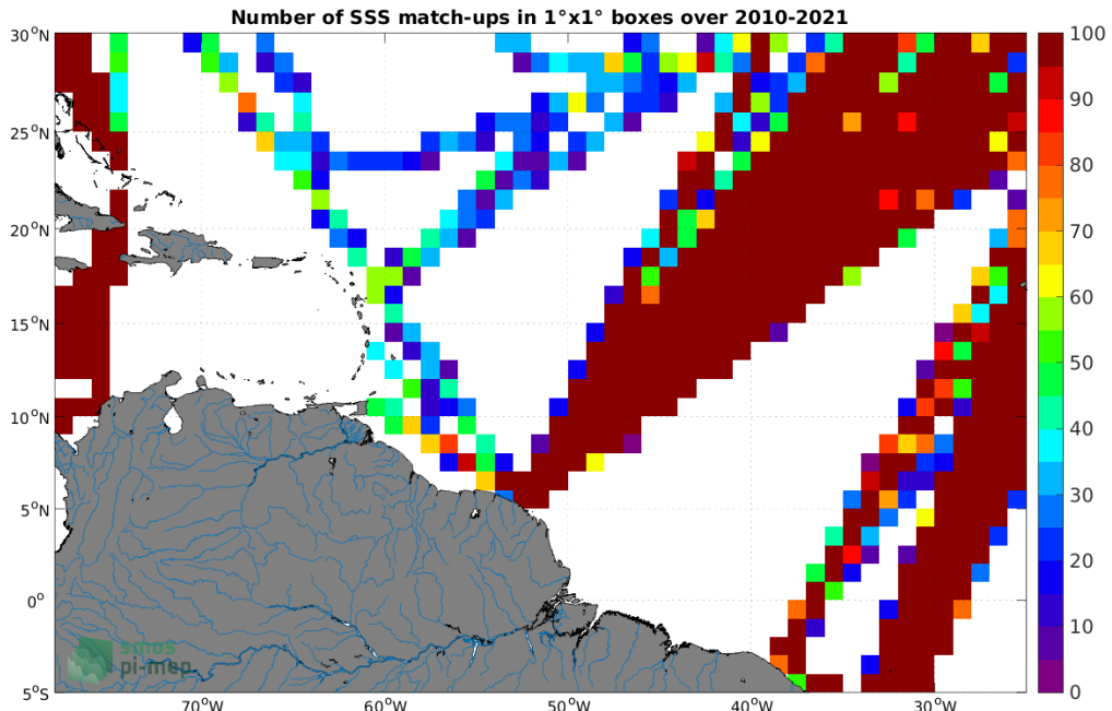
Figure 4: Number of SSS match-ups between TSG (LEGOS-DM) SSS and the SMOS SSS L3 v332 - 9 Days (CATDS-CPDC) SSS product for the Amazon and Orinoco river plumes Pi-MEP region over 1^\circ \times 1^\circ boxes and for the full satellite product period.
