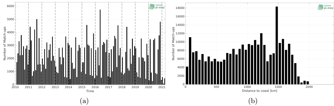
Figure 1: Number of match-ups between TSG (LEGOS-DM) and SMOS SSS L3 v332 - 9 Days (CATDS-CPDC) SSS as a function of time (a) and as function of the distance to coast (b) over the Amazon and Orinoco river plumes Pi-MEP region and for the full satellite product period.
