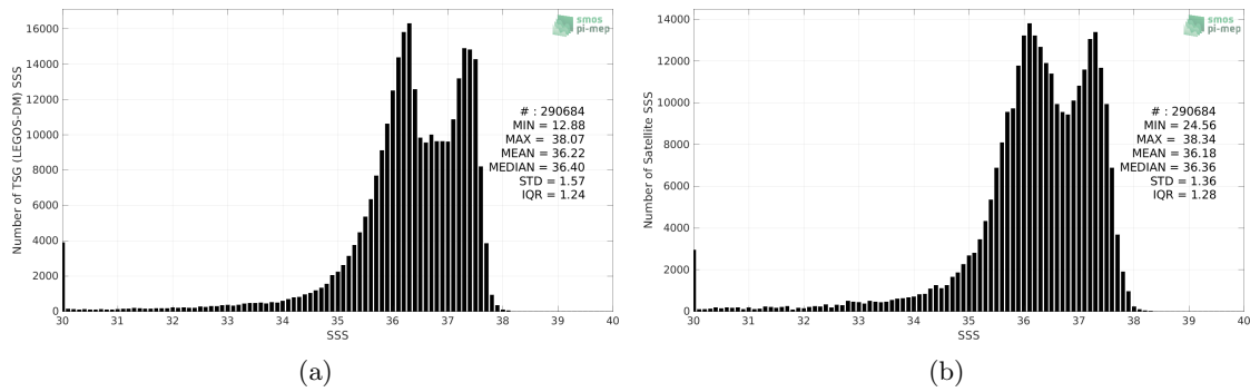
Figure 2: Histograms of SSS from TSG (LEGOS-DM) (a) and SMOS SSS L3 v332 - 9 Days (CATDS-CPDC) (b) considering all match-up pairs per bins of 0.1 over the Amazon and Orinoco river plumes Pi-MEP region and for the full satellite product period.
