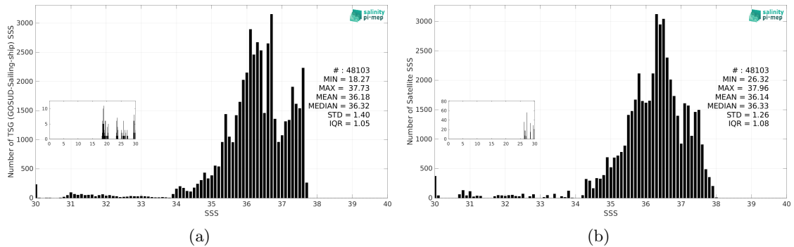
Figure 3: Histograms of SSS from TSG (GOSUD-Sailing-ship) (a) and SMOS SSS L3 v332 - 9 Days (CATDS-CPDC) (b) considering all match-up pairs per bins of 0.1 over the Amazon and Orinoco river plumes Pi-MEP region and for the full satellite product period.
