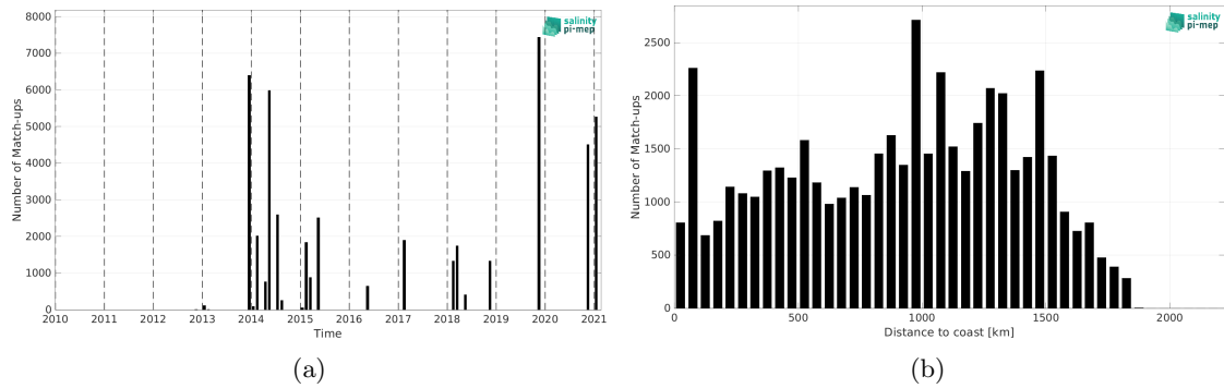
Figure 1: Number of match-ups between TSG (GOSUD-Sailing-ship) and SMOS SSS L3 v332 - 9 Days (CATDS-CPDC) SSS as a function of time (a) and as function of the distance to coast (b) over the Amazon and Orinoco river plumes Pi-MEP region and for the full satellite product period.
