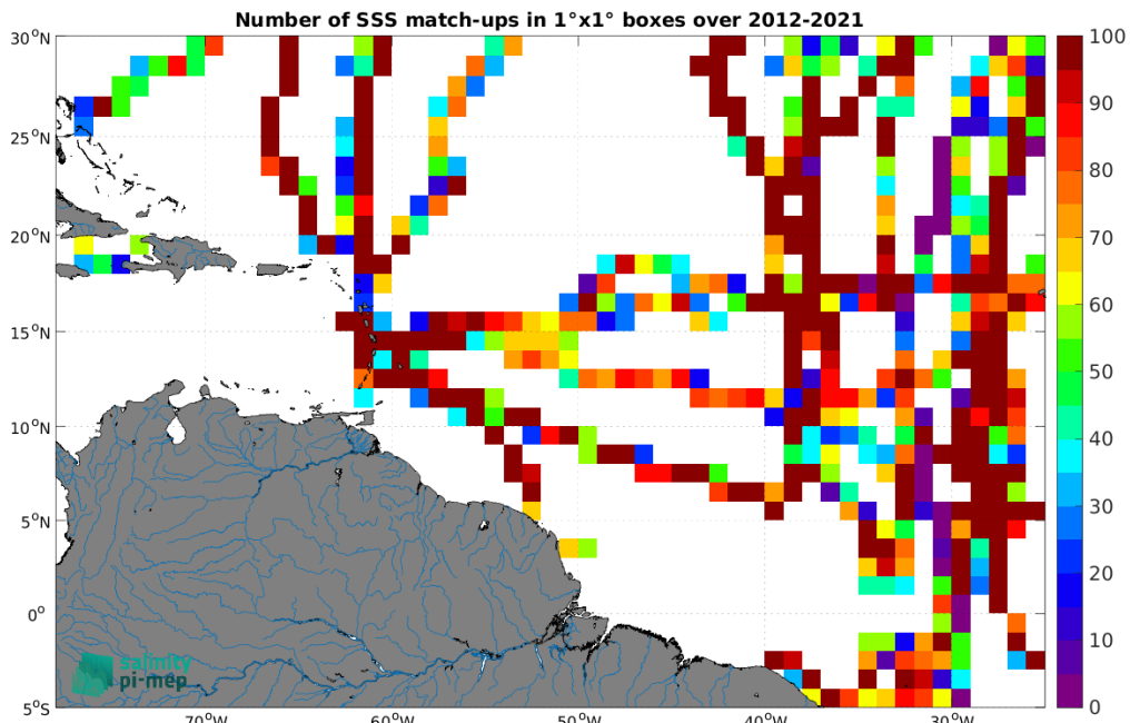
Figure 4: Number of SSS match-ups between TSG (GOSUD-Sailing-ship) SSS and the SMOS SSS L3 v332 - 9 Days (CATDS-CPDC) SSS product for the Amazon and Orinoco river plumes Pi-MEP region over 1^\circ \times 1^\circ boxes and for the full satellite product period.
