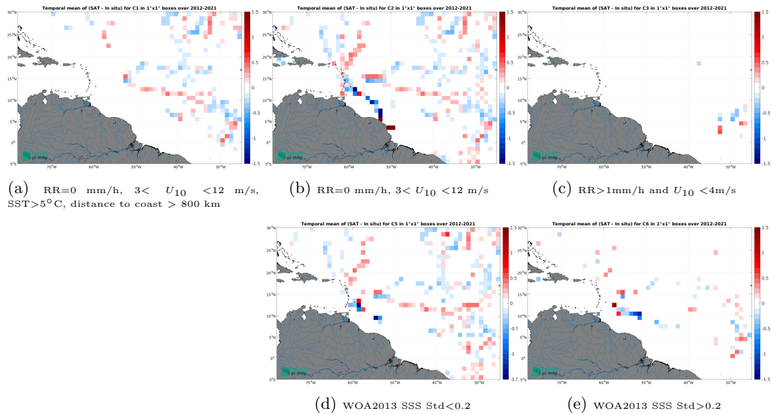
Figure 12: Temporal mean gridded over spatial boxes of size 1^{\circ}\times 1^{\circ} of \Delta SSS (SMOS SSS L3 v332 - 9 Days (CATDS-CPDC) - TSG (GOSUD-Sailing-ship)) for 5 different subdatasets corresponding to:RR=0 mm/h, 3 < U_{10} < 12 m/s, SST >5^{\circ}\text{C} , distance to coast > 800 km (a), RR=0 mm/h, 3 < U_{10} < 12 m/s (b), RR >1 mm/h and U_{10} < 4 m/s (c), WOA2013 SSS Std <0.2 (d), WOA2013 SSS Std >0.2 (e).
