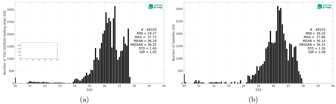
Figure 2: Histograms of SSS from TSG (GOSUD-Sailing-ship) (a) and SMOS SSS L3 v332 - 9 Days (CATDS-CPDC) (b) considering all match-up pairs per bins of 0.1 over the Amazon and Orinoco river plumes Pi-MEP region and for the full satellite product period.
