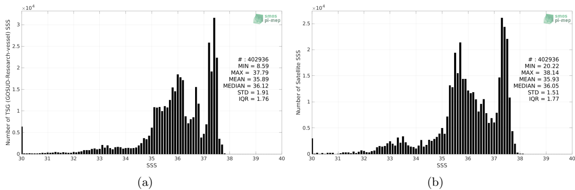
Figure 2: Histograms of SSS from TSG (GOSUD-Research-vessel) (a) and SMOS SSS L3 v332 - 9 Days (CATDS-CPDC) (b) considering all match-up pairs per bins of 0.1 over the Amazon and Orinoco river plumes Pi-MEP region and for the full satellite product period.
