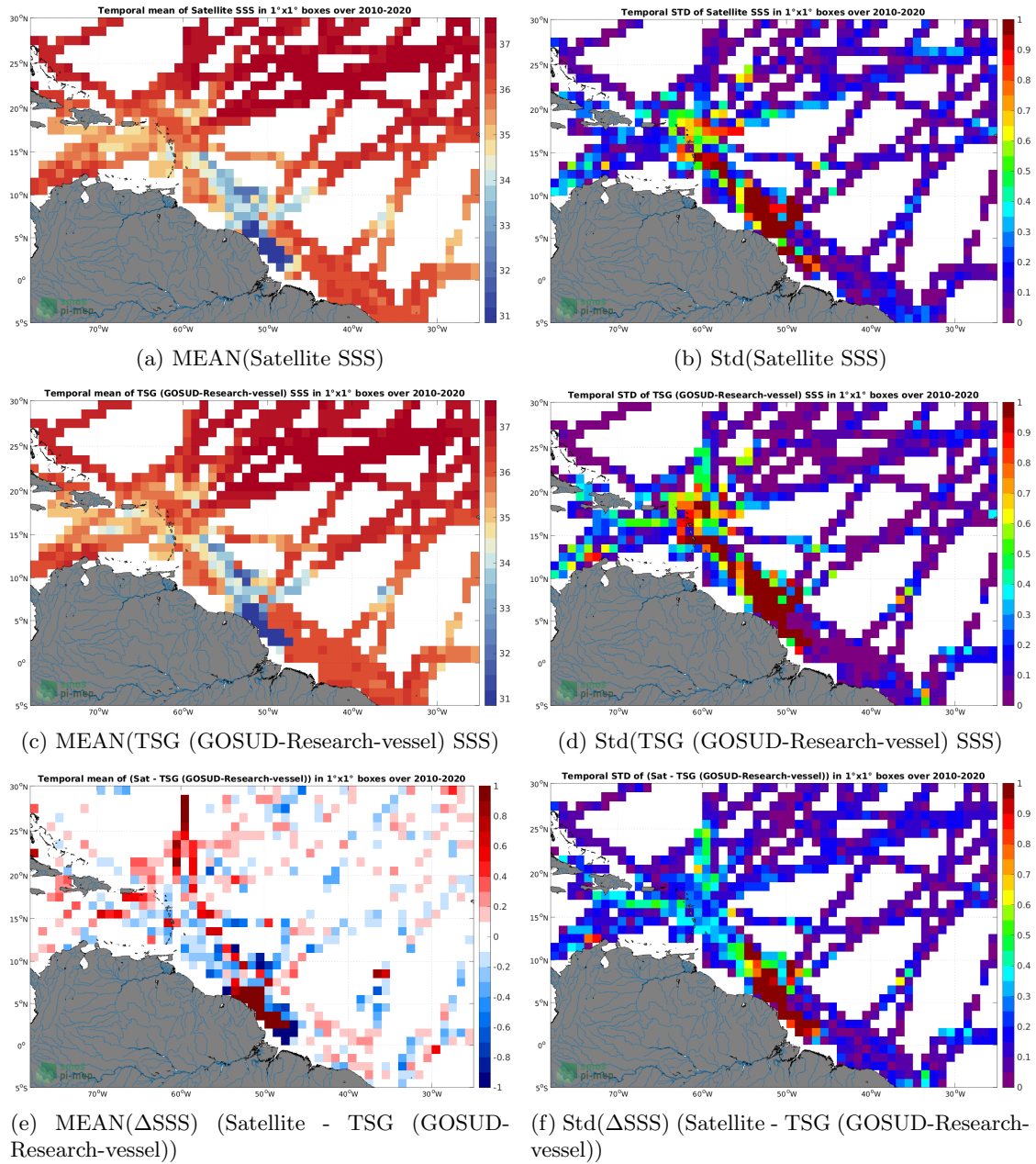
Figure 6: Temporal mean (left) and Std (right) of SSS from SMOS SSS L3 v332 - 9 Days (CATDS-CPDC) (top), TSG (GOSUD-Research-vessel) (middle), and of \Delta SSS (Satellite - TSG (GOSUD-Research-vessel)). Only match-up pairs are used to generate these maps.
