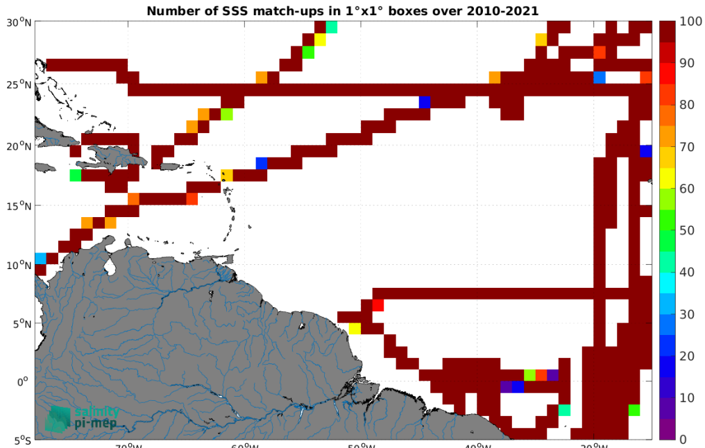
Figure 5: Number of SSS match-ups between TSG (CSIC-UTM) SSS and the SMOS SSS L3 v332 - 9 Days (CATDS-CPDC) SSS product for the Amazon and Orinoco river plumes Pi-MEP region over 1^\circ \times 1^\circ boxes and for the full satellite product period.
