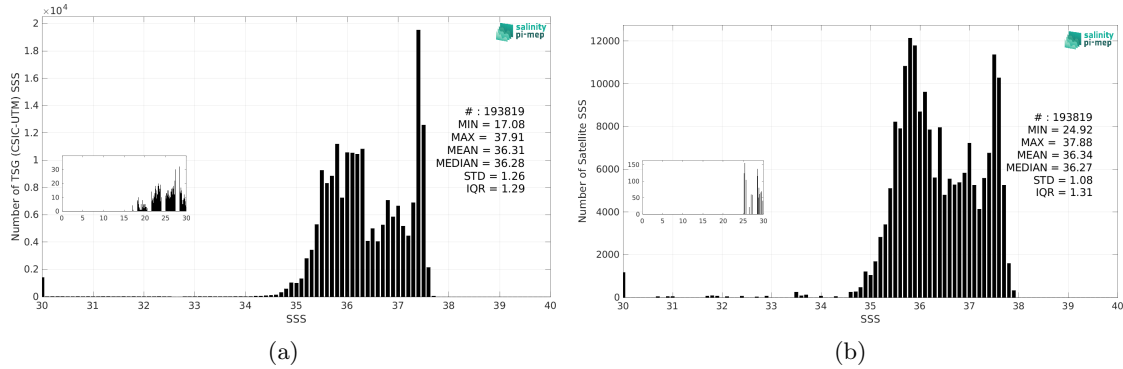
Figure 3: Histograms of SSS from TSG (CSIC-UTM) (a) and SMOS SSS L3 v332 - 9 Days (CATDS-CPDC) (b) considering all match-up pairs per bins of 0.1 over the Amazon and Orinoco river plumes Pi-MEP region and for the full satellite product period.
