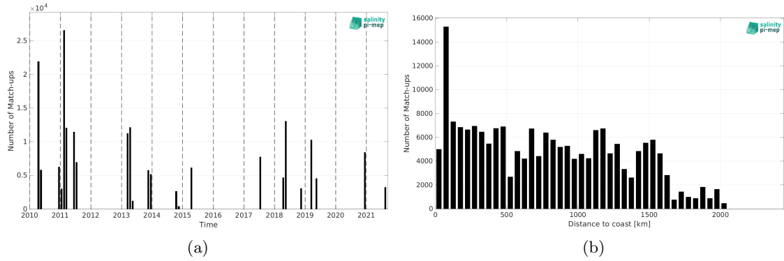
Figure 2: Number of match-ups between TSG (CSIC-UTM) and SMOS SSS L3 v332 - 9 Days (CATDS-CPDC) SSS as a function of time (a) and as function of the distance to coast (b) over the Amazon and Orinoco river plumes Pi-MEP region and for the full satellite product period.
