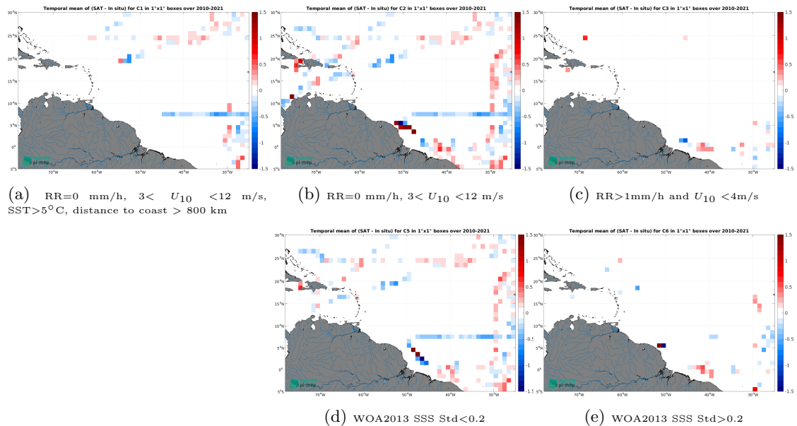
Figure 12: Temporal mean gridded over spatial boxes of size 1^\circ \times 1^\circ of \Delta SSS (SMOS SSS L3 v332 - 9 Days (CATDS-CPDC) - TSG (CSIC-UTM)) for 5 different subdatasets corresponding to:RR=0 mm/h, 3 < U_{10} < 12 m/s, SST >5^\circ C, distance to coast > 800 km (a), RR=0 mm/h, 3 < U_{10} < 12 m/s (b), RR >1 mm/h and U_{10} < 4 m/s (c), WOA2013 SSS Std <0.2 (d), WOA2013 SSS Std >0.2 (e).
