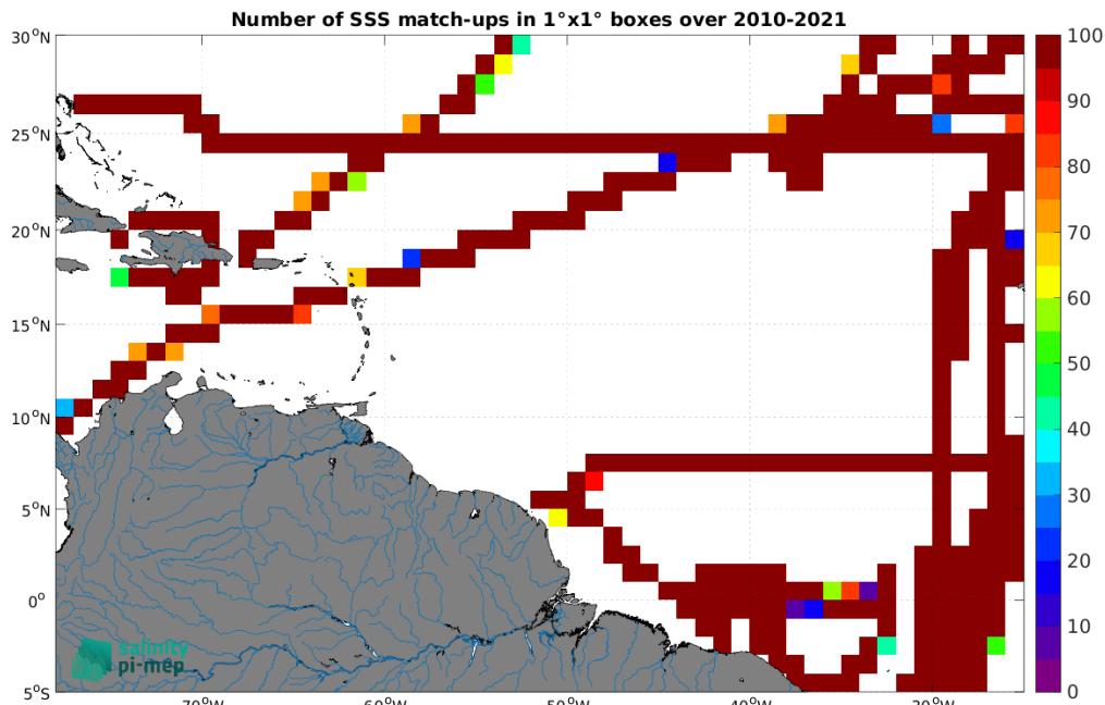
Figure 4: Number of SSS match-ups between TSG (CSIC-UTM) SSS and the SMOS SSS L3 v332 - 9 Days (CATDS-CPDC) SSS product for the Amazon and Orinoco river plumes Pi-MEP region over 1^\circ \times 1^\circ boxes and for the full satellite product period.
