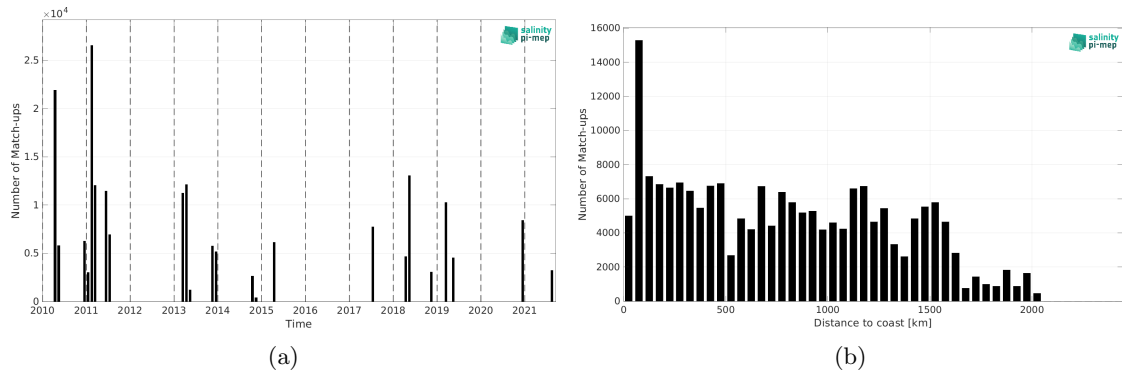
Figure 1: Number of match-ups between TSG (CSIC-UTM) and SMOS SSS L3 v332 - 9 Days (CATDS-CPDC) SSS as a function of time (a) and as function of the distance to coast (b) over the Amazon and Orinoco river plumes Pi-MEP region and for the full satellite product period.
