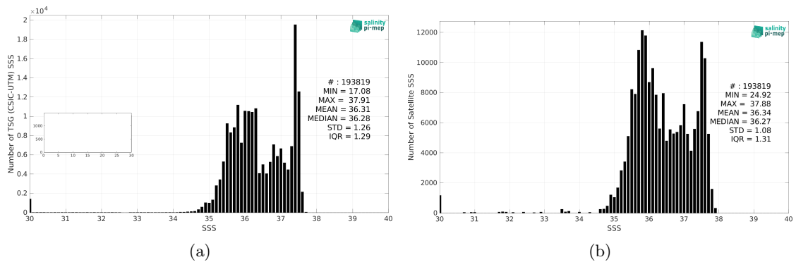
Figure 2: Histograms of SSS from TSG (CSIC-UTM) (a) and SMOS SSS L3 v332 - 9 Days (CATDS-CPDC) (b) considering all match-up pairs per bins of 0.1 over the Amazon and Orinoco river plumes Pi-MEP region and for the full satellite product period.
