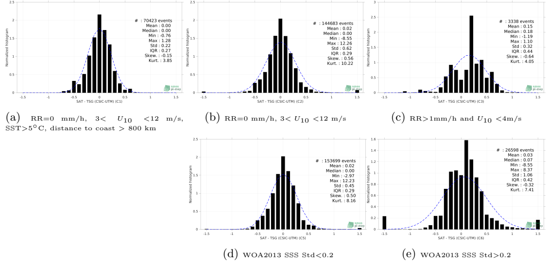
Figure 13: Normalized histogram of \Delta SSS (SMOS SSS L3 v332 - 9 Days (CATDS-CPDC) - TSG (CSIC-UTM)) for 5 different subdatasets corresponding to: RR=0 mm/h, 3 < U_{10} < 12 m/s, SST>5°C, distance to coast > 800 km (a), RR=0 mm/h, 3 < U_{10} < 12 m/s (b), RR>1mm/h and U_{10} < 4 m/s (c), WOA2013 SSS Std<0.2 (d), WOA2013 SSS Std>0.2 (e).
