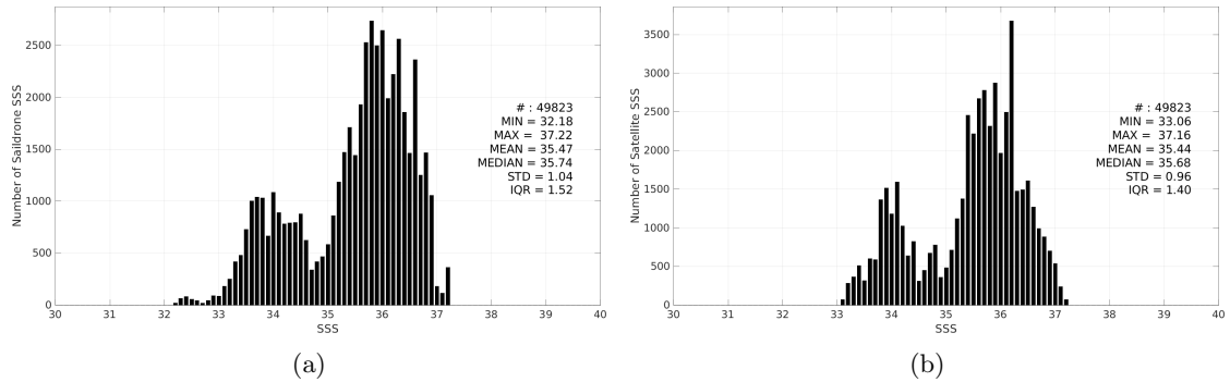
Figure 3: Histograms of SSS from Saildrone (a) and SMOS SSS L3 v332 - 9 Days (CATDS-CPDC) (b) considering all match-up pairs per bins of 0.1 over the Amazon and Orinoco river plumes Pi-MEP region and for the full satellite product period.
