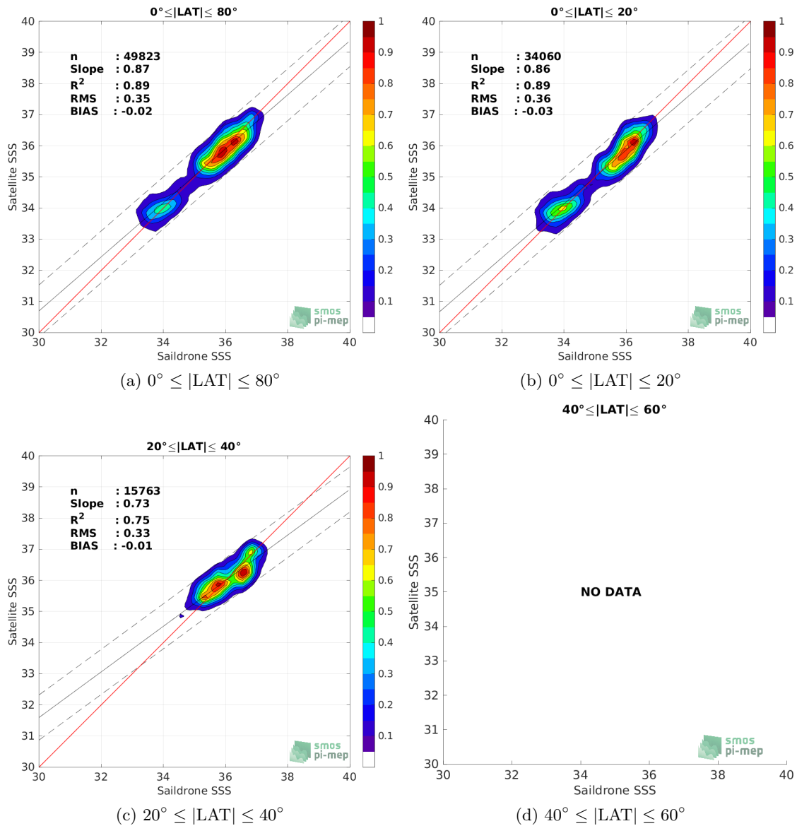
Figure 9: Contour maps of the concentration of SMOS SSS L3 v332 - 9 Days (CATDS-CPDC) SSS (y-axis) versus Sailldrone SSS (x-axis) at match-up pairs for different latitude bands. For each plot, the red line shows x=y . The black thin and dashed lines indicate a linear fit through the data cloud and the \pm 95\% confidence levels, respectively. The number match-up pairs n , the slope and R^2 coefficient of the linear fit, the root mean square (RMS) and the mean bias between satellite and in situ data are indicated for each latitude band in each plots.
