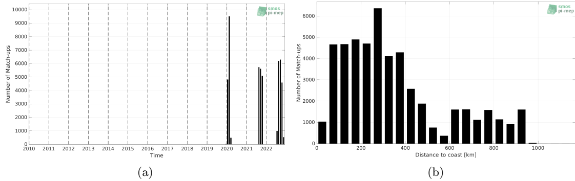
Figure 1: Number of match-ups between Saïdrone and SMOS SSS L3 v332 - 9 Days (CATDS-CPDC) SSS as a function of time (a) and as function of the distance to coast (b) over the Amazon and Orinoco river plumes Pi-MEP region and for the full satellite product period.
