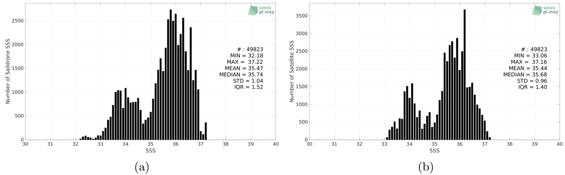
Figure 2: Histograms of SSS from Saïdrone (a) and SMOS SSS L3 v332 - 9 Days (CATDS-CPDC) (b) considering all match-up pairs per bins of 0.1 over the Amazon and Orinoco river plumes Pi-MEP region and for the full satellite product period.
