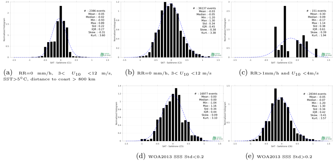
Figure 13: Normalized histogram of \Delta SSS (SMOS SSS L3 v332 - 9 Days (CATDS-CPDC) - Saildrone) for 5 different subdatasets corresponding to: RR=0 mm/h, 3 < U_{10} < 12 m/s, SST > 5^\circ C , distance to coast > 800 km (a), RR=0 mm/h, 3 < U_{10} < 12 m/s (b), RR > 1 mm/h and U_{10} < 4 m/s (c), WOA2013 SSS Std < 0.2 (d), WOA2013 SSS Std > 0.2 (e).
